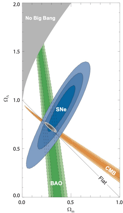
FIG. 6: From [32]: 68.3 %, 95.4 % and 99.7% Confidence level contours on \Omega_\Lambda \equiv \Omega_{DE} and \Omega_m obtained from CMB, BAO and the Union SN set ( P/\rho \equiv w = -1 ). This is “Concordance Cosmology”: The contributions of the cosmological constant \Omega_\Lambda and of the (ordinary + dark) matter \Omega_m to the ratio total density/critical density, i.e. , the density for which the universe is spatially flat, are yielded (modulo their uncertainty ranges) through Supernovae (SNe), Baryonic Acoustic Oscillations (BAO), and Cosmic Microwave Radiation (CMB). One sees that alternative models to Big Bang (No Big Bang) are excluded. The straight line \Omega_\Lambda + \Omega_m = 1 which is marked “flat” corresponds to a spatially flat Universe.
