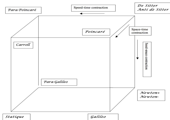
FIG. 1: The eleven kinematics (Bacry & Levy-Leblond, JMP (1968)). From [12].
