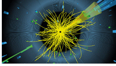
FIG. 5: From Strong interactions News: Protons probe quark-gluon plasma at CMS , 13 January 2017.
