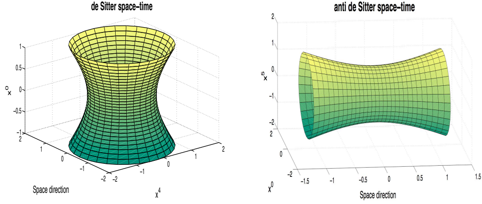
FIG. 2: Left: the one-sheeted de Sitter hyperboloid as a manifold embedded in the 1 + 4 Minkowski space-time. x^0 might be chosen as a time parameter, but there is no global time-like Killing vector. Right: the one-sheeted Anti de Sitter hyperboloid as a manifold embedded in the 2 + 3 ambient space. Angular position along the central belt can be chosen as a local time coordinate, and it is in one-to-one correspondence with a global time-like Killing vector.
