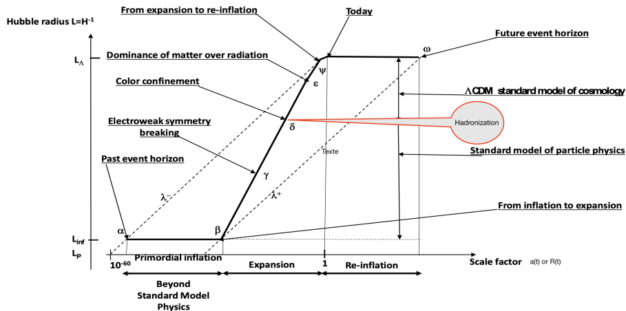
FIG. 4: Cosmology chronology: Hubble radius L(a) \equiv H^{-1}(a) ( c = 1 ) is plotted versus the scale factor a(t) \equiv R(t) in logarithmic scale. (from [7])
