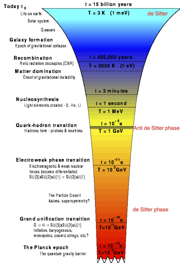
FIG. 3: Cosmology chronology (from http://zebu.uoregon.edu/images/bb_history.gif ).
