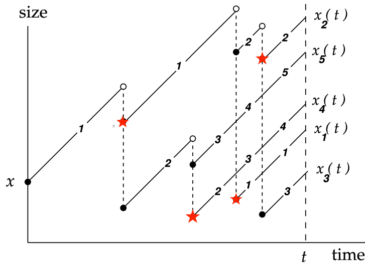
FIG 2. Same example as in Figure 1, with n_t = 5 . The cells at time t have sizes (x_j(t))_{j=1,2,\dots,5} . At each time of cell division, two marks appear: a (red) star and a dot. The heights of these two marks represent the sizes of the two daughter cells: if the parent-cell has index k , then the star corresponds to the child-cell with index k and the dot corresponds to the child-cell with index k + 1 . Note that according to our way of labelling the cell numbers, cells may change their index without splitting.
