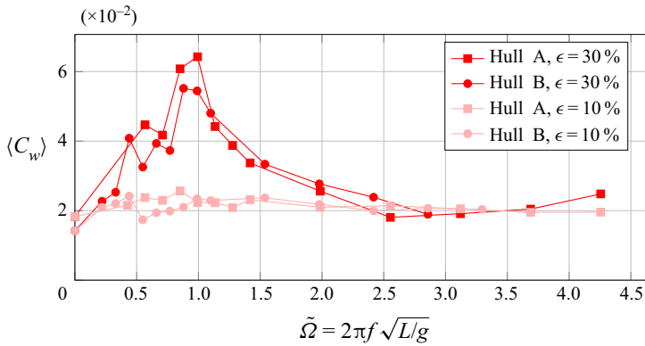
Figure 15. Mean wave drag coefficient \langle C_w \rangle = \langle R_w \rangle / (0.5\rho V^{2/3} V_0^2) as a function of the fluctuation frequency, at \mathcal{F}_0 = 0.3 . Hulls A and B differ by a geometric three-dimensional scaling factor of 5/3.
