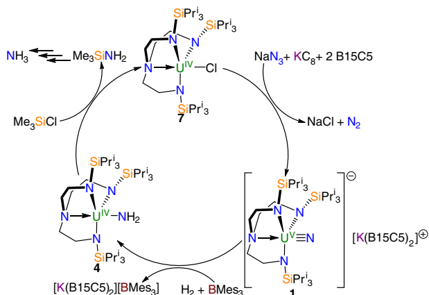
Fig. 8 Reaction cycle for the production of ammonia. Treatment of 7 with sodium azide, \text{KC}_8 , and two equivalents of B15C5 produces the terminal uranium-nitride 1 , which in turn reacts with \text{H}_2 and \text{BMes}_3 to give 4 . Treatment of 4 with \text{Me}_3\text{SiCl} , followed by work-up and acidification steps, as indicated by the multiple arrows, produces ammonia. B15C5 = benzo-15-crown-5 ether. Mes = 2,4,6-trimethylphenyl.
