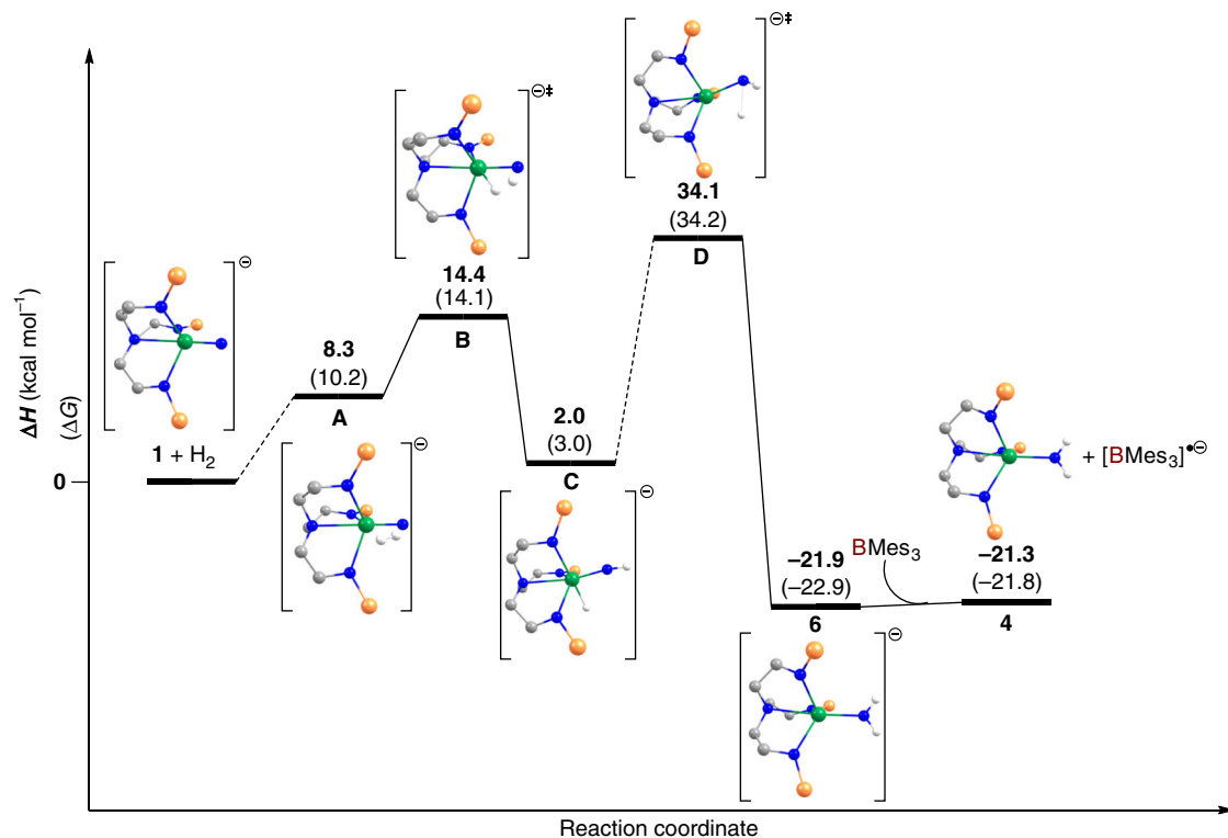
Fig. 9 Computed reaction profile for the conversion of 1 to 6 in the absence of \text{BMes}_3 and then conversion to 4 with the addition of \text{BMes}_3 . The isopropyl groups of the silyl substituents, carbon-bound hydrogen atoms, and [\text{K}(\text{B15C5}_2)]^+ cation accommodated in the calculations are omitted for clarity. Bold numbers without parentheses refer to \Delta H values and numbers in parentheses are \Delta G values, both quoted in \text{kcal mol}^{-1} .
