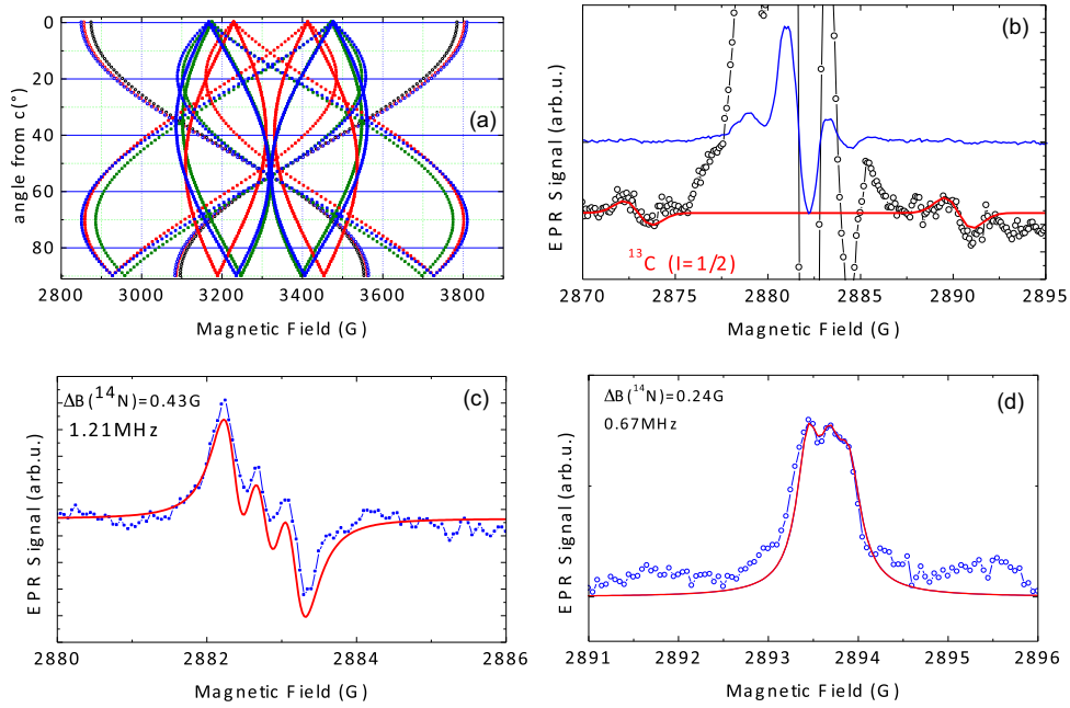
FIG. 4. EPR spectra of the NV^- centers at T = 4 K under nonresonant excitation displaying the six NV^- centers. (a) Angular variation of the six NV centers for a rotation of the magnetic field from B//c to B//[11-20] , allowing the determination of the spin Hamiltonian parameters compiled in Table II. (b) For the highest-intensity axial NV center ( k2k1 ) the central hyperfine interaction with one ^{13}C nucleus (one of the three C neighbors) is resolved (blue); (red line): spectrum multiplied by 200. (c) Higher resolution EPR spectrum of the axial NV center ( k1k2 ) displaying directly the SHF interaction with nuclear spin I = 1 of the ^{14}N neighbor. (d) EPR spectrum of the hk1 basal NV center showing a strongly reduced SHF with ^{14}N as compared to the other NV centers.
