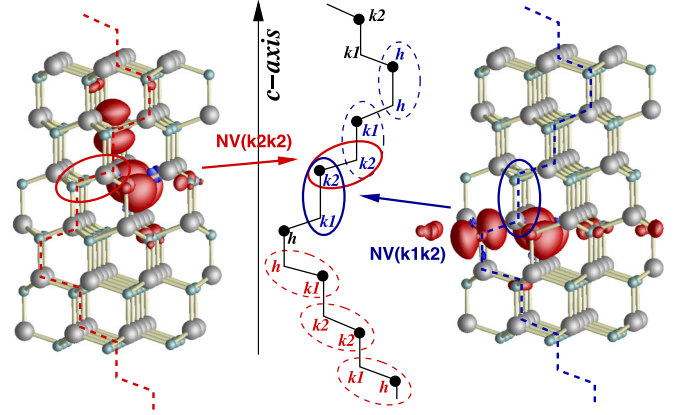
FIG. 1. Crystal structure of 6H-SiC showing the three nonequivalent Si and C (black circles) lattice sites, hexagonal ( h ) and quasicubic ( k1 and k2 ), whereby k1 is always neighboring one k2 and three h sites ( k2 has quasicubic neighbors exclusively). Thus we obtain the following NV center configurations: basal : hk1 , k2k2 , k1h and axial : hh , k2k1 , k1k2 (for further details see the text). As an example we show also the magnetization density of the basal ( k2k2 , left) and the axial ( k1k2 , right) NV pair providing C_{1h} and C_{3v} symmetry, respectively.
