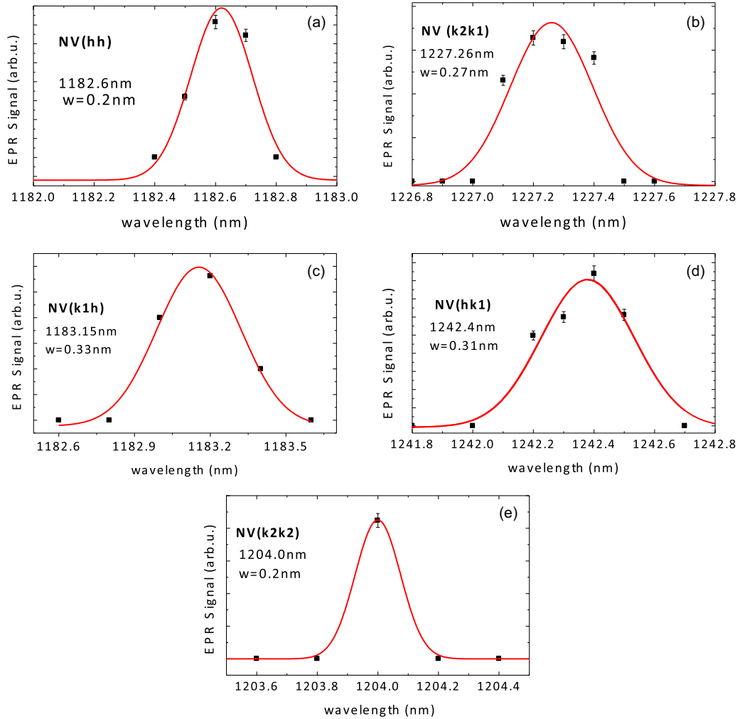
FIG. 6. (a)–(e) Resonant excitation EPR spectra measured (at T = 4 K) individually for each \text{NV}^- center on its low field EPR line. These spectra correspond to the ZPL absorption lines of the NV centers; the ZPL expected at 1155 nm is out of range of the tunable NIR laser but can be attributed from the knowledge of the other five ZPL lines.
