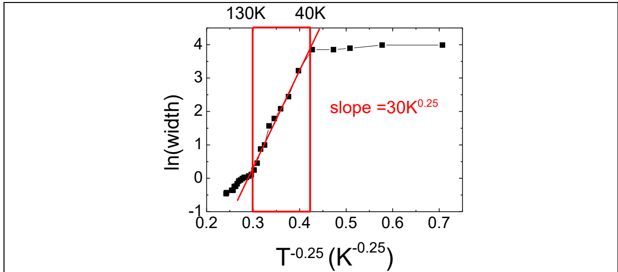
Figure 5: Mott plot of the linewidth \ln(\Delta B) as a function of temperature T^{-0.25} in the as-received sample
