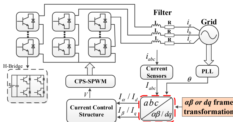
Figure 1. Block diagram of cascaded H-bridge grid-connected inverter.
