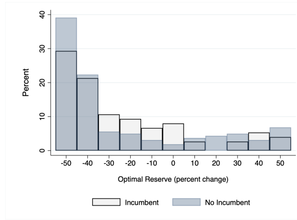
Figure 1: Histogram of the Optimal Reserve
