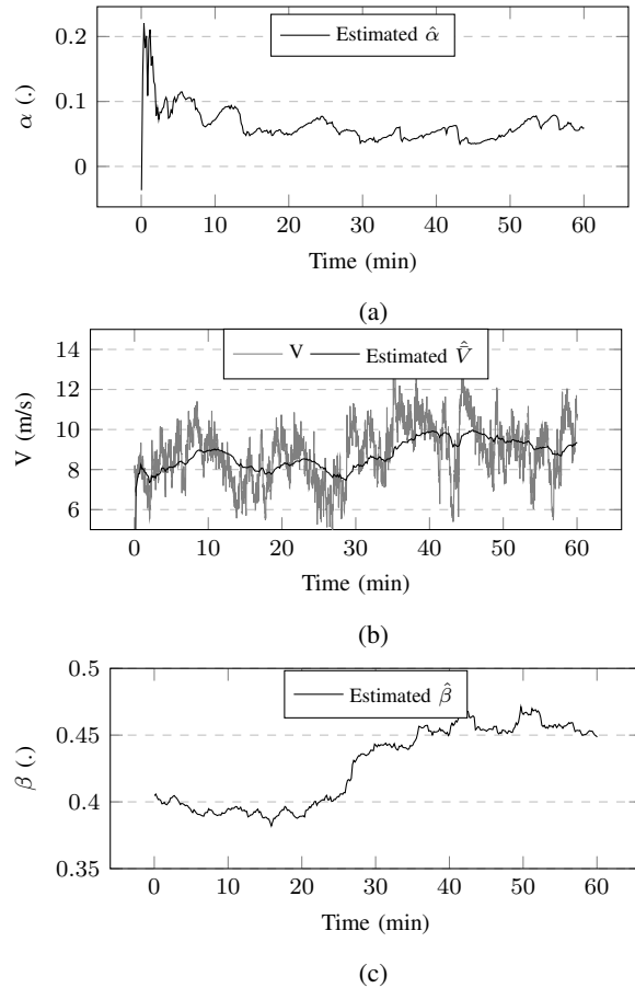
Fig. 4: Estimation of OU parameters (a) \hat{\alpha} (b) \hat{V} and (c) \hat{\beta} of real measured wind data.
