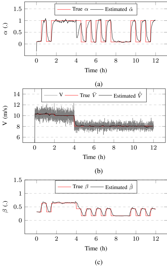
Fig. 3: Estimation of OU parameters (a) \hat{\alpha} (b) \hat{V} and (c) \hat{\beta} of generated wind data using [10].
