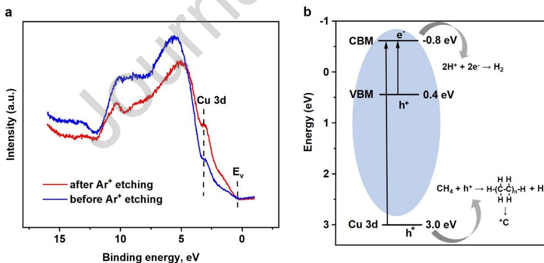
Figure 7. (a) UPS spectra acquired for an as-grown CIGS sample and after \text{Ar}^+ treatment for 10 minutes at an energy of 1 keV. The positions of the Cu 3d like-states and the Fermi level are indicated with vertical segments. (b) Band levels and elementary steps in methane coupling.
