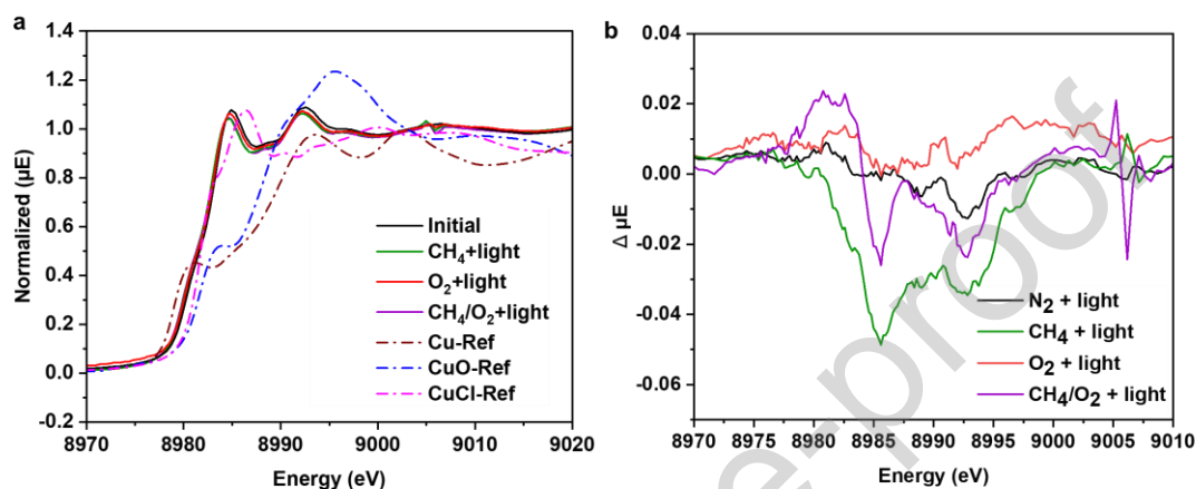
Figure 4. In-situ Cu K-edge XANES spectra of CIGS after N 2 , CH 4 , O 2 and CH 4 /O 2 treatment in comparison with reference samples (a) and the difference between these samples and initial spectrum (b).
