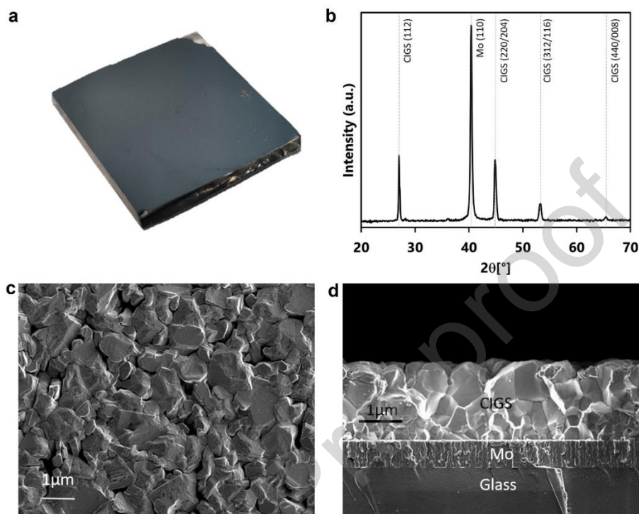
Figure 2. (a) Image of CIGS coated plate 2 \times 2 \text{ cm}^2 , (b) XRD pattern of CIGS, SEM analysis of CIGS layer coating: (c) top view and (d) cross-section.
