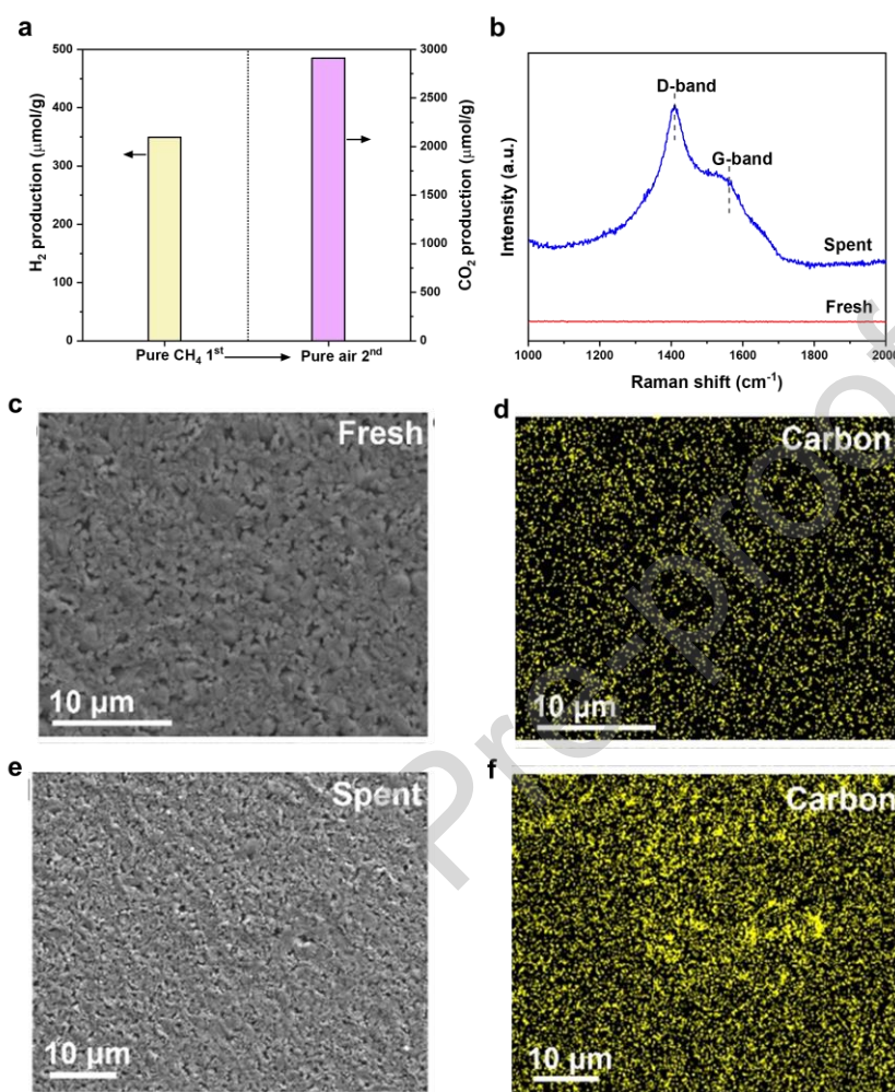
Figure 6. (a) Photocatalytic performance of CIGS plate under sequential pure \text{CH}_4 and air conditions. Reaction condition: 2 mg catalyst, 20^\circ\text{C} , 5 bar, 15h irradiation. (b) Raman spectra of fresh and spent CIGS plate. SEM and EDX-mapping images of carbon over fresh (c,d) and spent CIGS plate (e,f). Note that the spent CIGS plate underwent the same treatment in pure \text{CH}_4 atmosphere as mentioned above.
