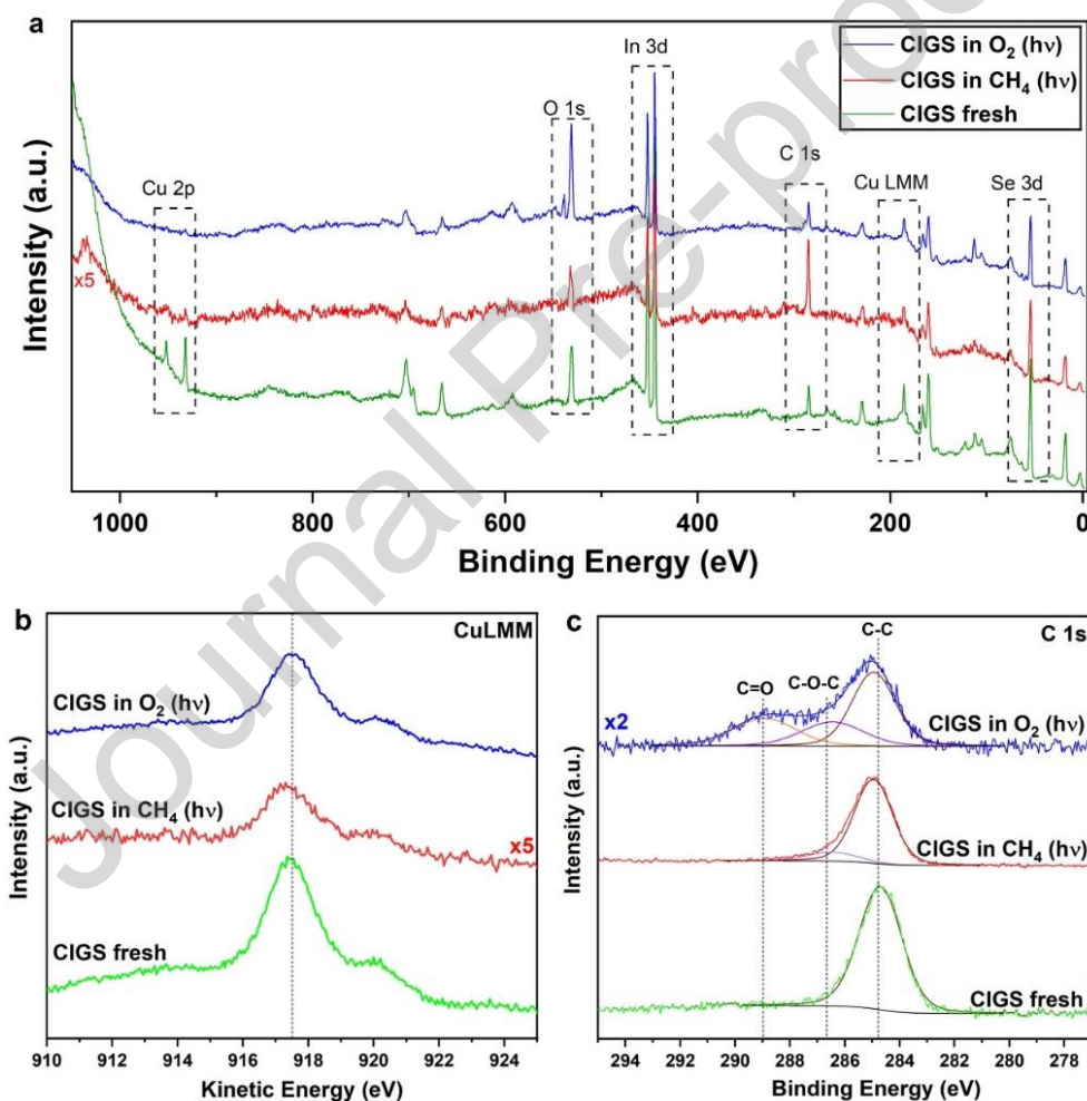
Figure 5. In-situ XPS normalized spectra of CIGS under different conditions (a) survey spectra; (b) Cu L 2,3 M 4,5 M 4,5 spectra; (c) C 1s spectra.
