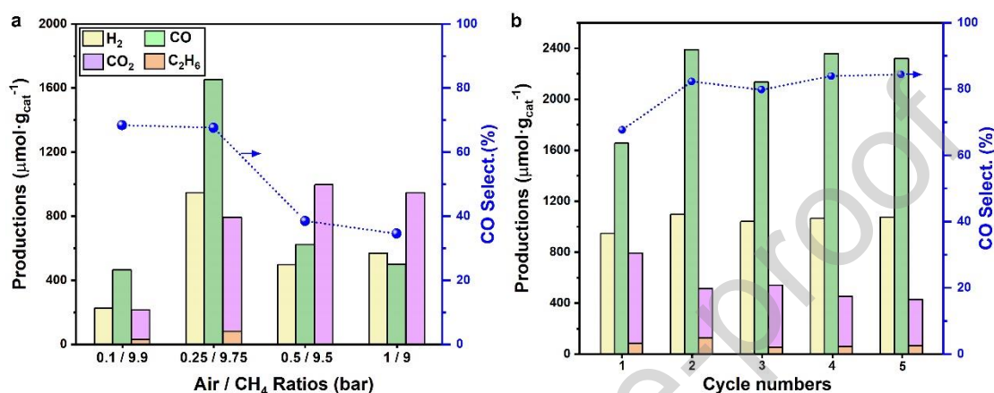
Figure 3. (a) Photocatalytic performance of CIGS sample under different air/CH 4 ratios. (b) Stability test of CIGS samples in 5 cyclic tests. Reaction conditions: 2 mg catalyst, 250 mL reactor, 20 °C, 15 h, a 400 W Hg-Xe lamp as the light source.
