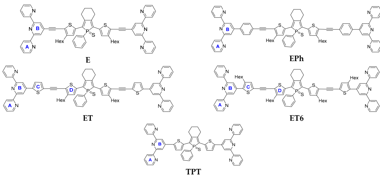
Scheme 1. Structures of the prepared new unimers (abbreviations derived from the names of linkers connecting tpy groups to the central unit) and the reference TPT unimer. (Adapted from ref. [19]).
