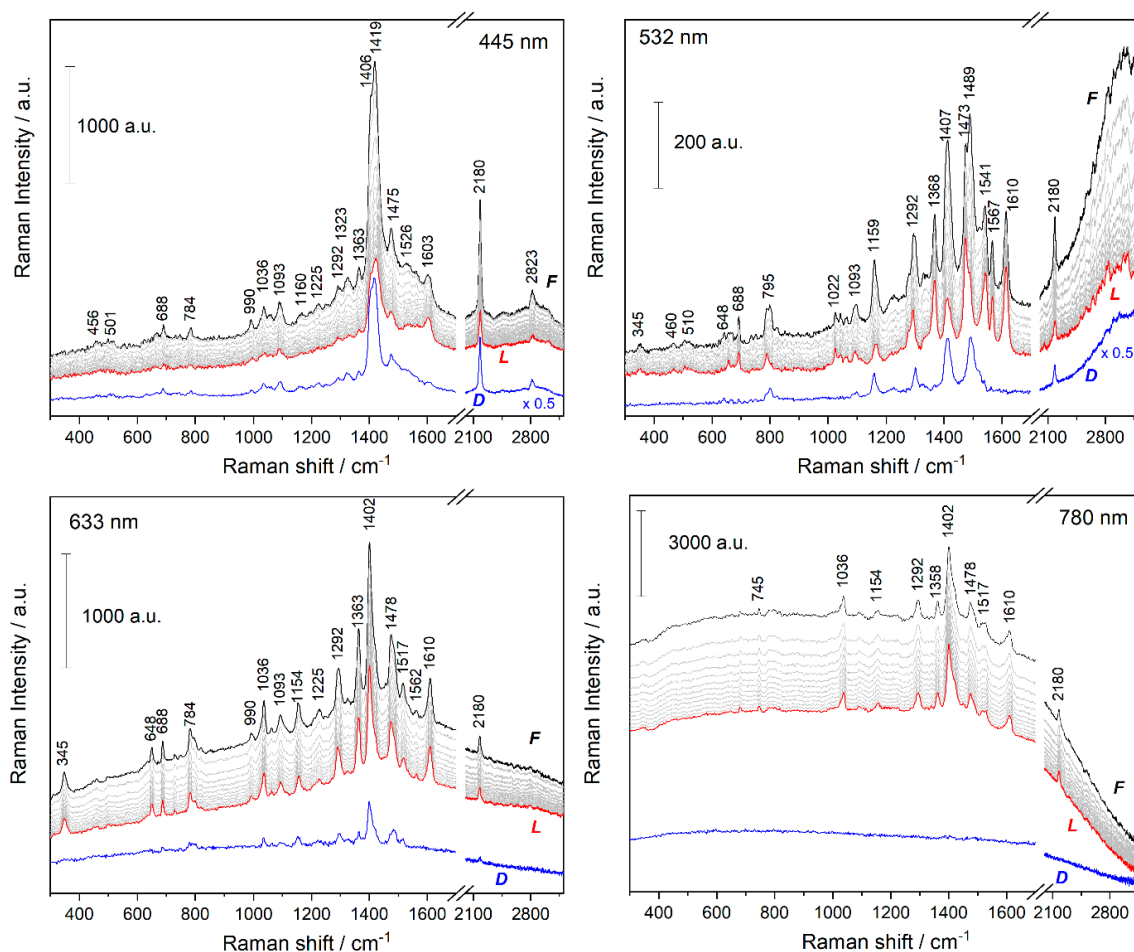
Figure 4. Time evolutions of the Raman spectra of FeET films measured using various \lambda_{exc} . Black—first RS ( F ); red—last measured RS ( L ); blue ( D = F - L )—difference spectrum. Accumulation time 15 s; total time 6–9 min; laser power at the sample: 0.1 mW for 532 and 633 nm and 5 mW for 445 and 780 nm.
