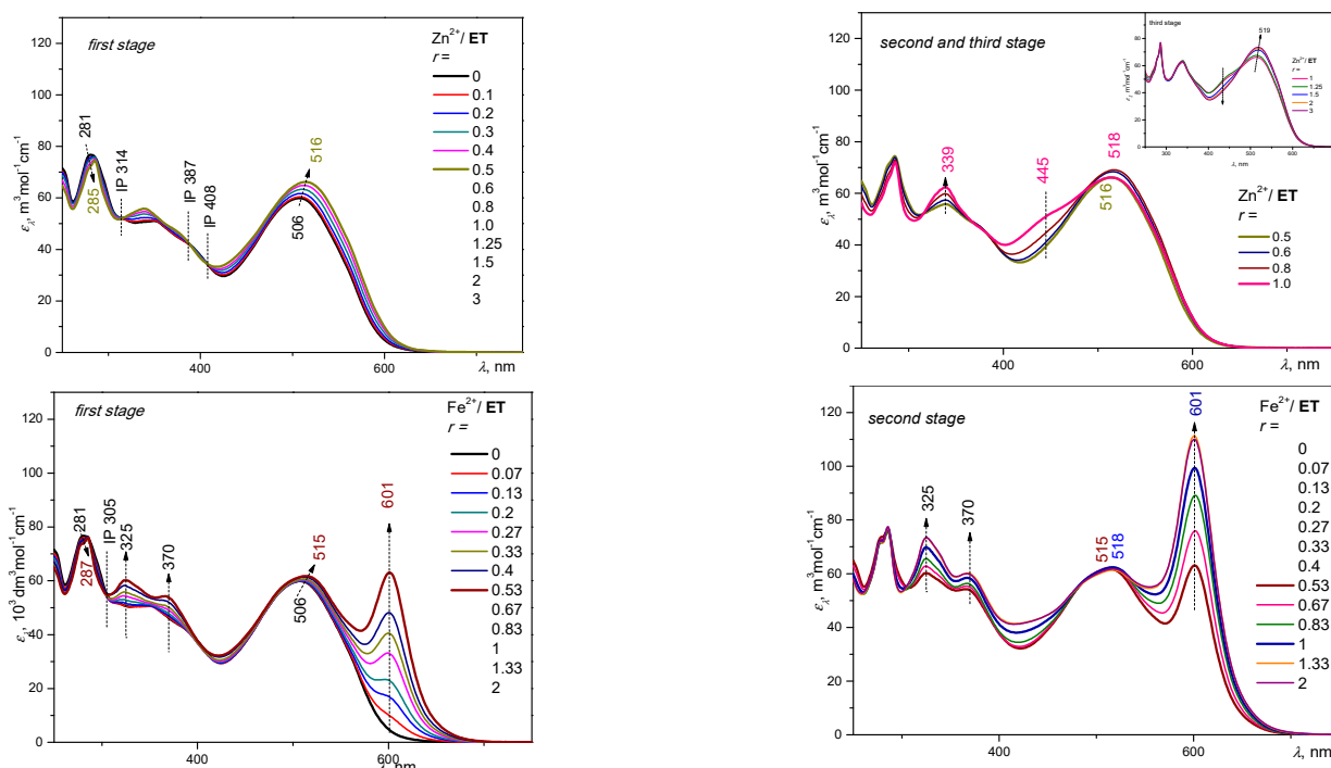
Figure 1. The UV/vis spectral changes accompanying assembly of \text{Zn}^{2+} (up) and \text{Fe}^{2+} (down) ions with unimer ET at mole ratios r from 0 to ca 0.5 (left) and at r > 0.5 (right).
