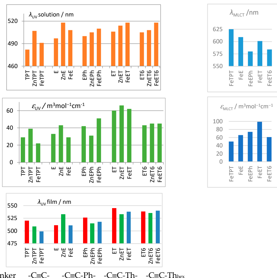
Figure 2. Effect of the linker structure on the UV/vis characteristics of unimers and MSPs.
