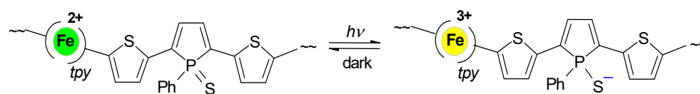
Scheme 3. Probable chemical nature of the observed phenomenon. \sim\sim indicating continuation of polymer chain.
