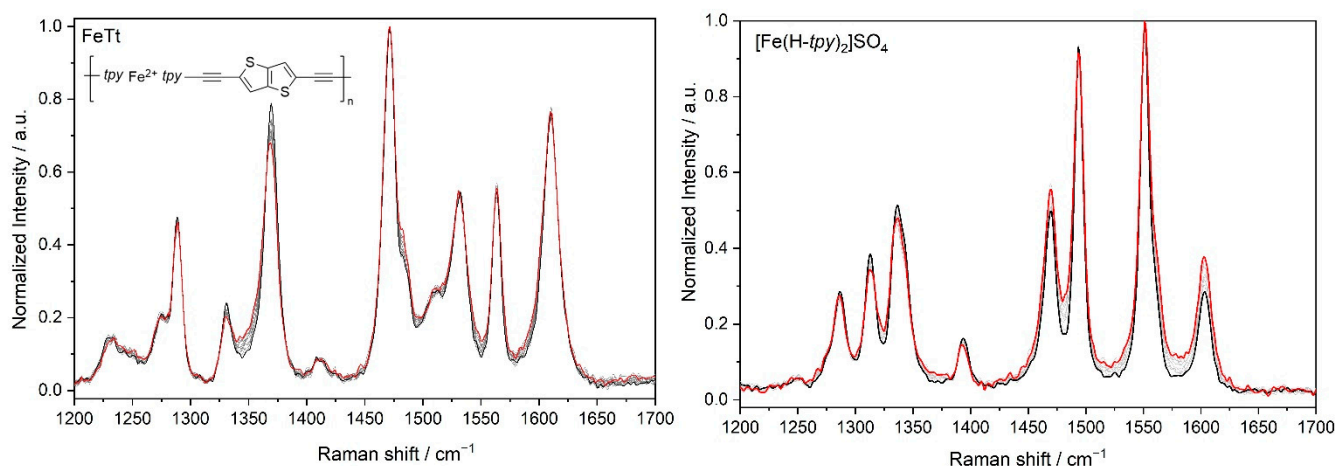
Figure 10. Overlaid baseline-corrected spectra of spectral sets of indicated compounds, normalized to the highest spectral band. Laser (532 nm) power 0.2 mW; accumulation 10 s; total time 9 min.
