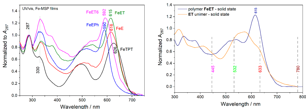
Figure 3. (Left): UV/vis spectra of Fe-MSP films. (Right): UV/vis spectra of films of the ET unimer and FeET polymer with the marked positions of the laser-beam wavelengths used for the excitation of Raman spectra.
