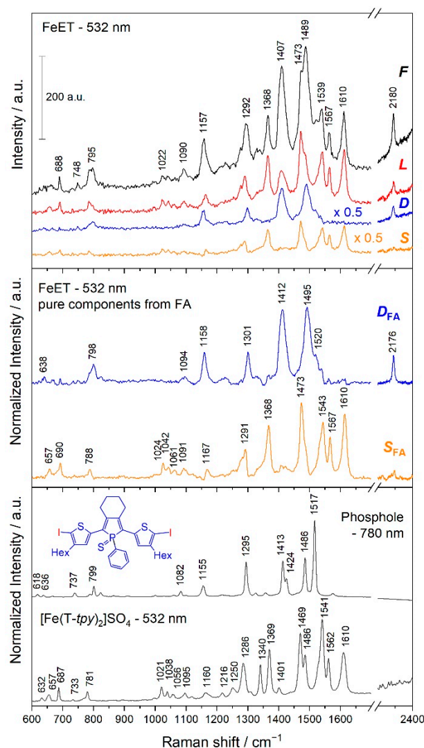
Figure 5. Comparison of relevant RS: ( Top ): the first ( F ) and last ( L ) RS of the FeET (532 nm) series and RSs of the disappearing ( D ) and stable ( S ) components obtained by the subtraction method; ( Middle ): pure spectral components obtained by factor analysis (FA) of the whole spectral set; ( Bottom ): off-resonance RS of the precursor central unit and RRS of [\text{Fe}(\text{T-tpy})_2]\text{SO}_4 complex (T-tpy stands for 4'-(2-thienyl)terpyridine).
