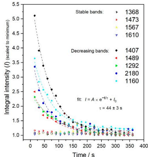
Figure 7. Time evolution of individual Raman bands of FeET exposed to the excitation radiation.
