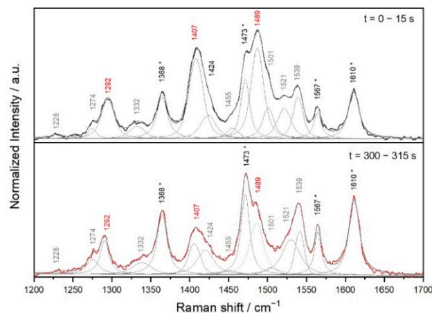
Figure 6. Deconvolution of the first and last RRS of FeET ( \lambda_{\text{exc}} = 532 nm; 0.1 mW).
