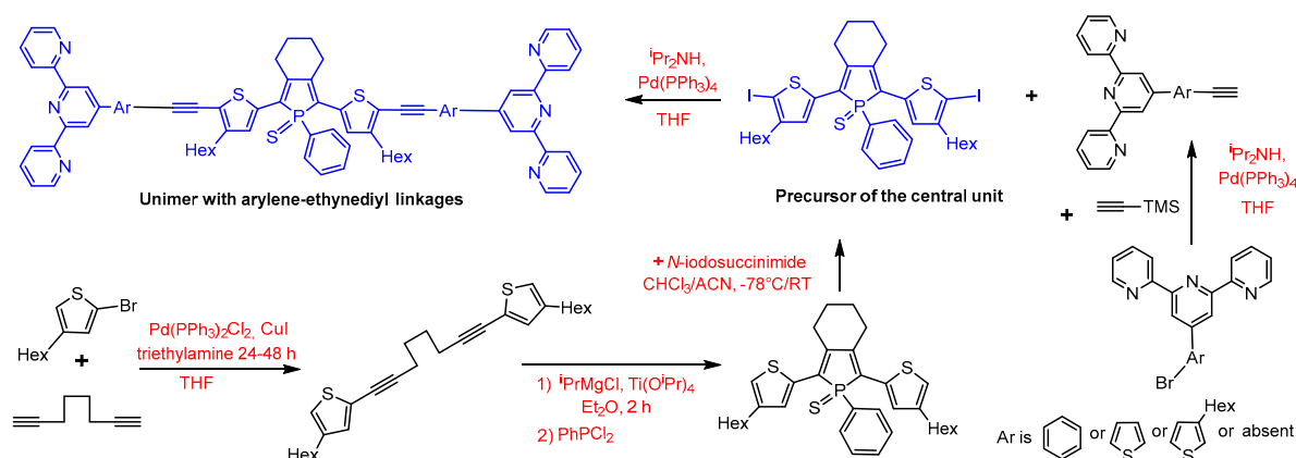
Scheme 2. Synthetic pathway to unimers.
