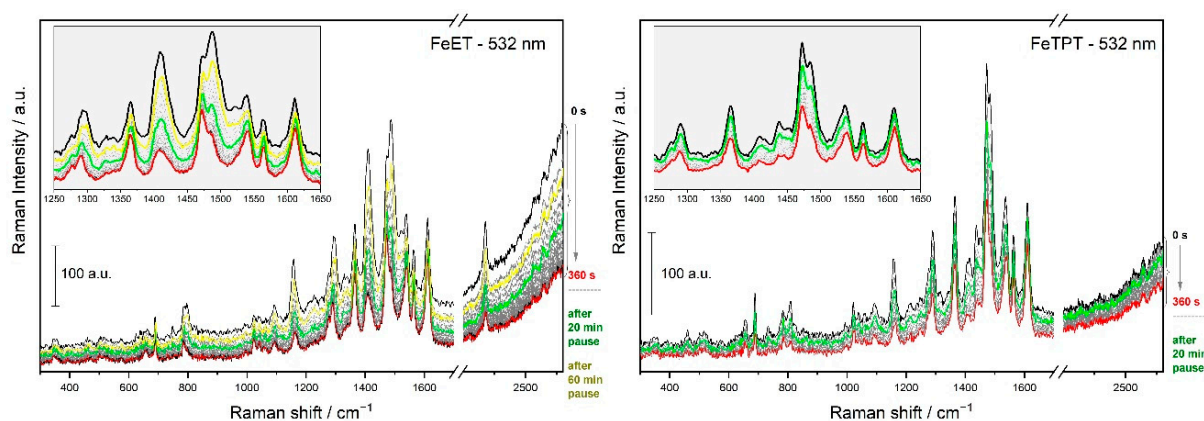
Figure 8. Tests of the reversibility of spectral changes for FeET and TPT. Black—first measured RRS; red—last measured RRS; green—RRS taken after 20 min pause; yellow—RRS taken after 60 min pause. Insets—details of the central parts of RRSs. Laser power 0.1 mW; accumulation time 15 s; total time 6 min.
