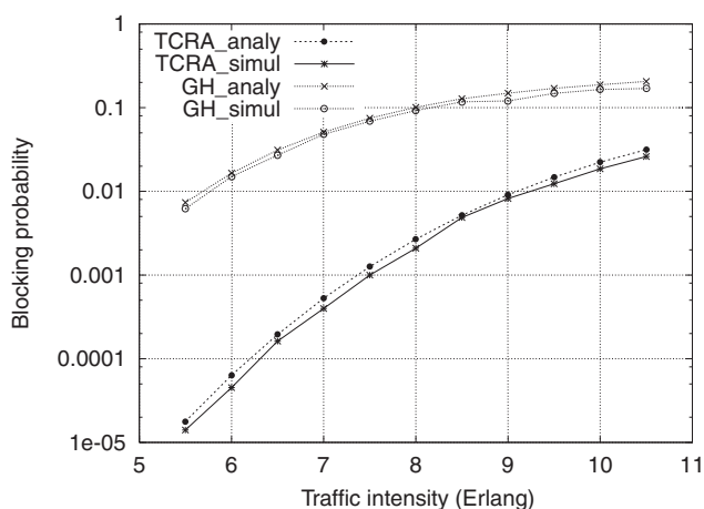
Fig. 3. Call blocking probabilities for TCRA and GH schemes
