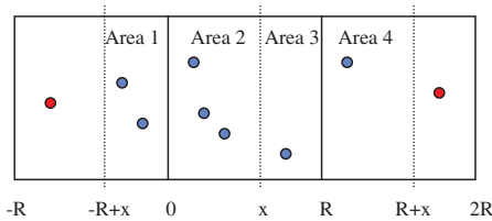
Fig. 2. Derivation of the blocking probability
