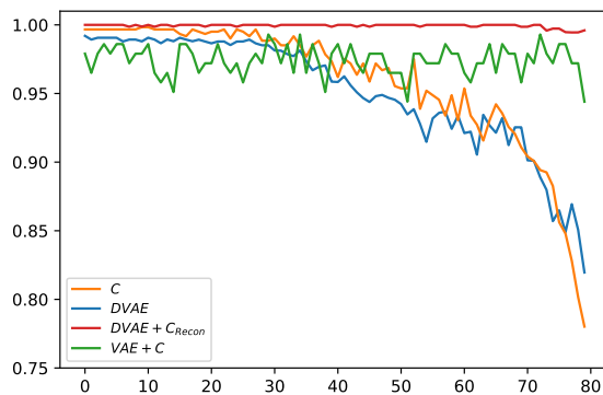
Fig. 6 Classification accuracy obtained with different methods in the presence of missing data. The x-axis corresponds to the percentage of missing data ( \times 100 ).
