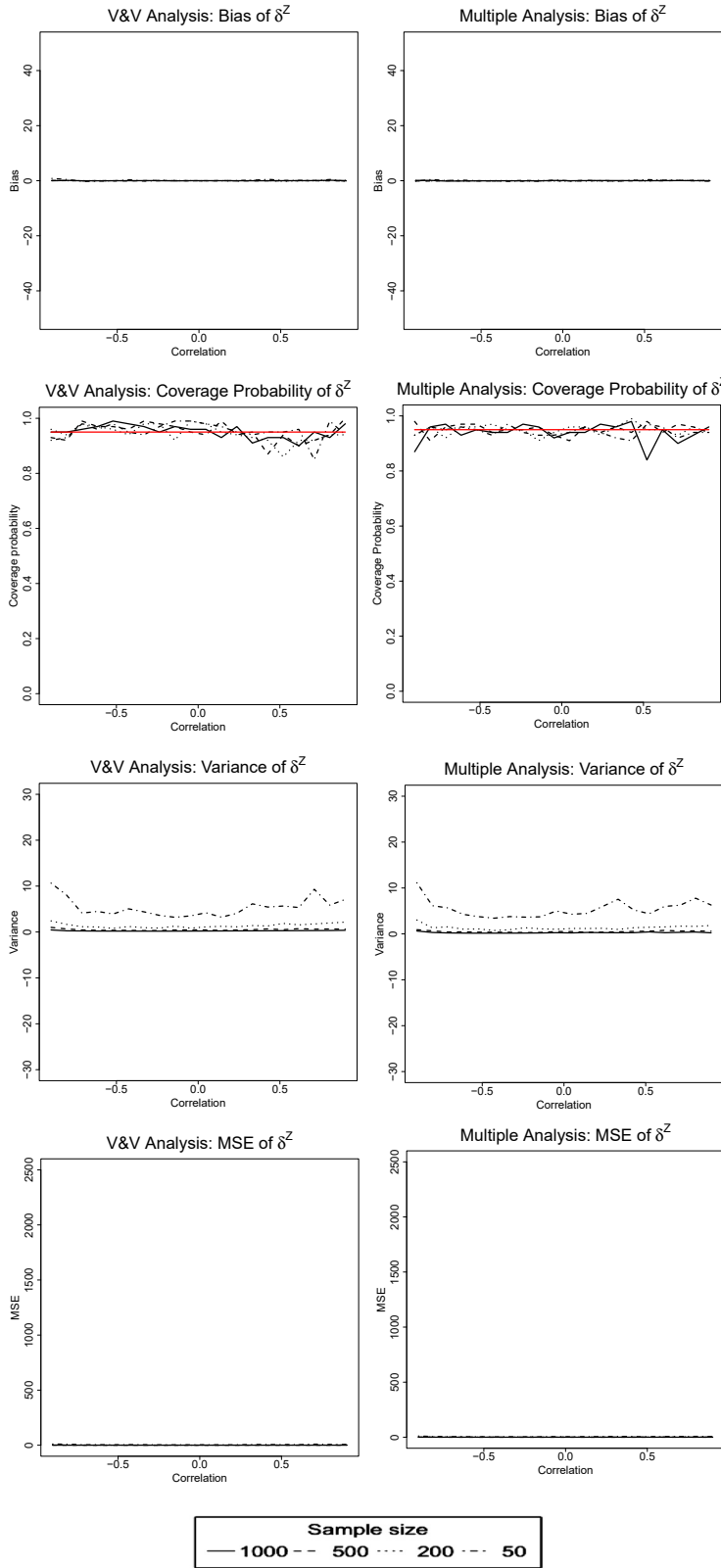
Figure 10: Model 1 (continuous outcome): bias, confidence interval coverage probability, mean square error (MSE), and variance of the joint direct effect estimator \delta^Z calculated as means over 200 simulation runs when the correlation between mediators varies. The bias formula used here is Bias = \theta - \mathbb{E}[\hat{\theta}] .
