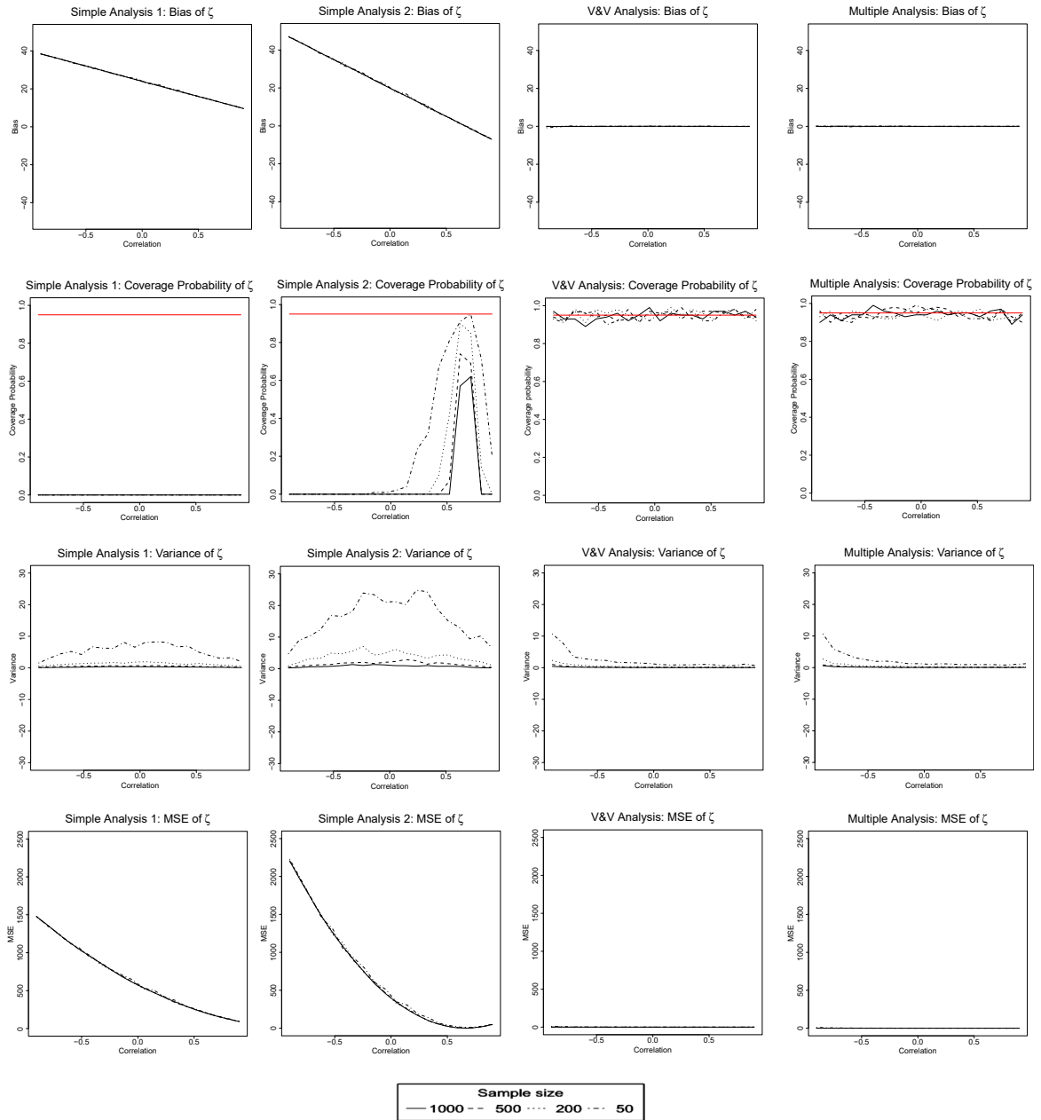
Figure 9: Model 1 (continuous outcome): bias, confidence interval coverage probability, mean square error (MSE), and variance of the direct effect estimator \zeta calculated as means over 200 simulation runs when the correlation between mediators varies. The bias formula used here is Bias = \theta - \mathbb{E}[\hat{\theta}] .
