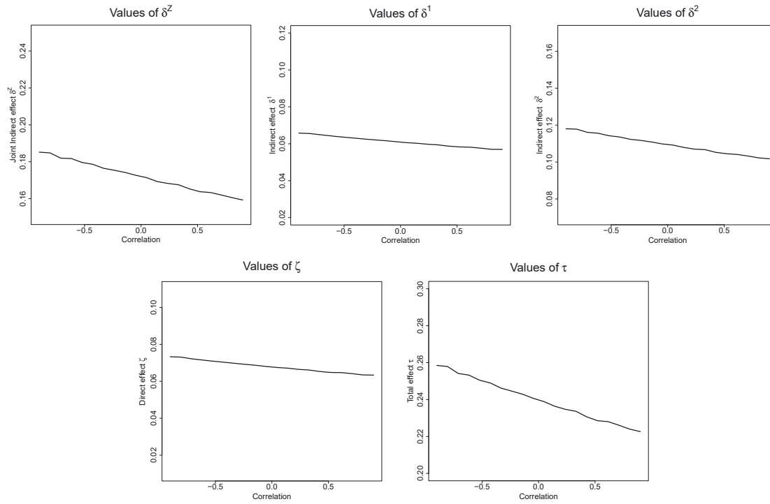
Figure 12: Binary outcome (model 2): variation in causal effects due to correlation.
