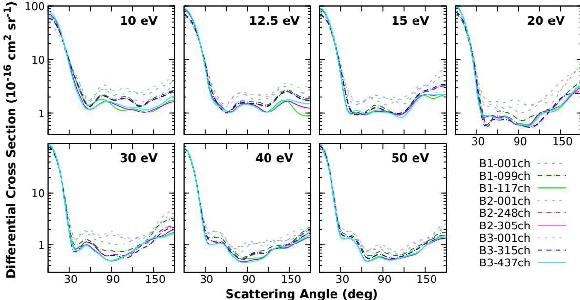
FIG. 5. Elastic differential cross sections for electron scattering from benzene, according to our nine scattering calculations. The B1-117ch and B2-315ch results were first reported in Ref. [33].
