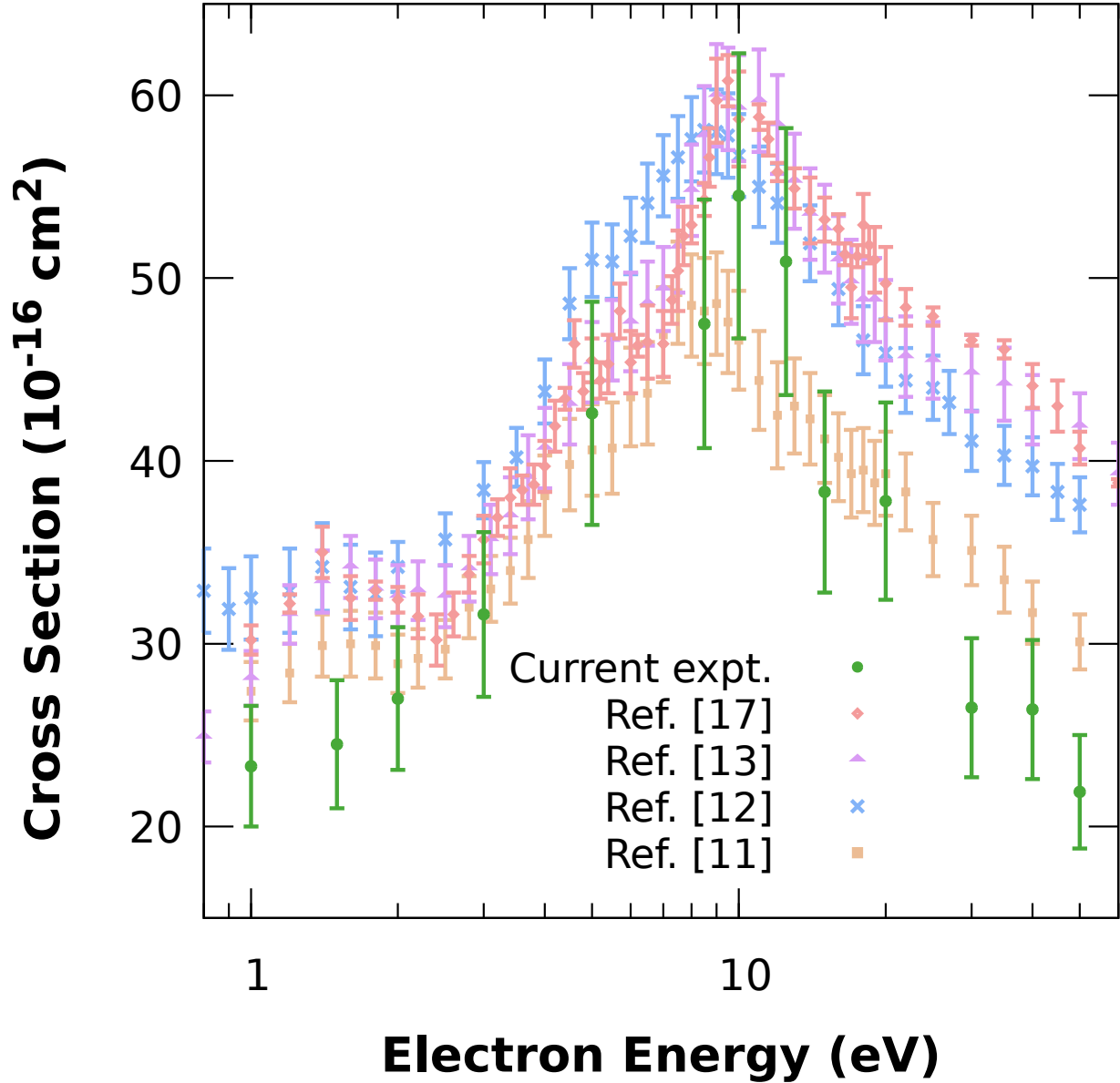
FIG. 7. Present measured elastic integral cross sections and available total cross sections as measured by Sueoka [11], Mozejko et al. [12], Makochehanwa et al. [13] and Costa et al. [17].
