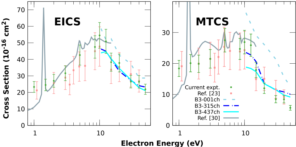
FIG. 6. Elastic integral and momentum transfer cross sections, EICS and MTCS, for electron scattering from benzene, according to the current measurements and previous ones from Cho et al. [23], together with the present calculations with the B3 basis set and three multichannel coupling schemes for the intermediate energies, and the theoretical results from Barbosa and Bettega [30] for the lower energies.
