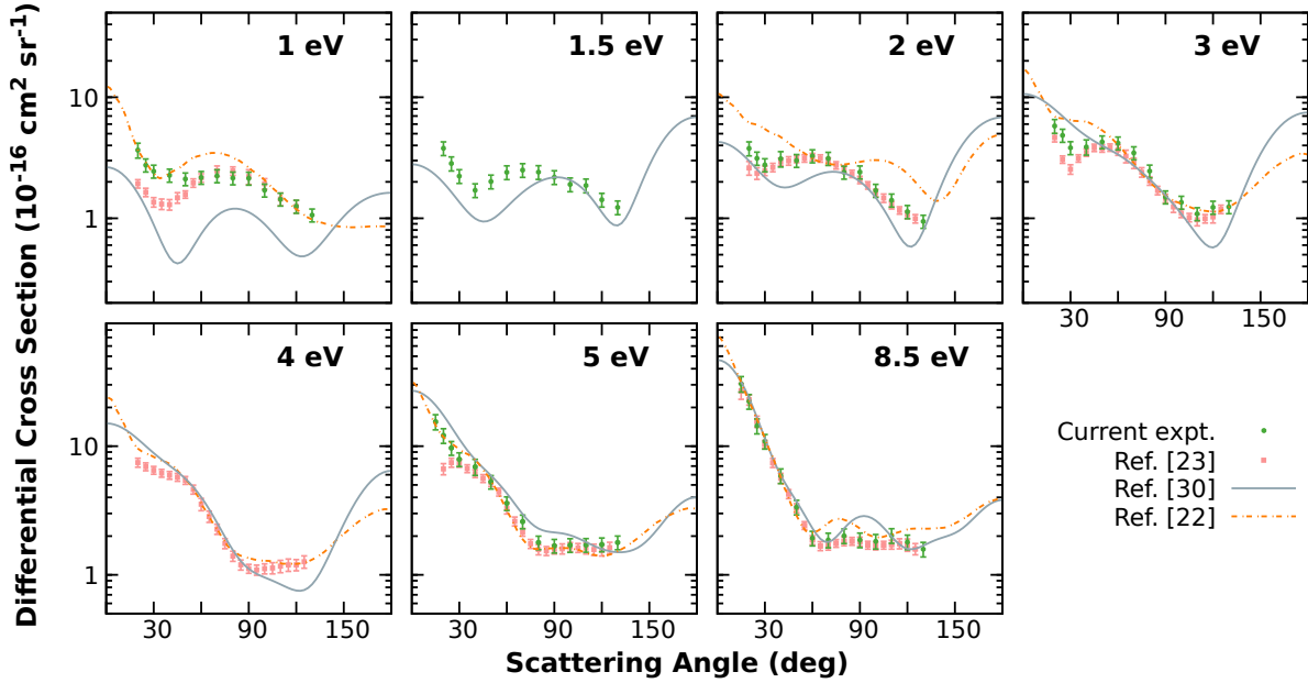
FIG. 3. Elastic differential cross sections for electron scattering from benzene, according to the current measurements and previous ones from Cho et al. [23], as well as to calculations reported by Barbosa and Bettega [30] and by Gianturco and Lucchese [22].
