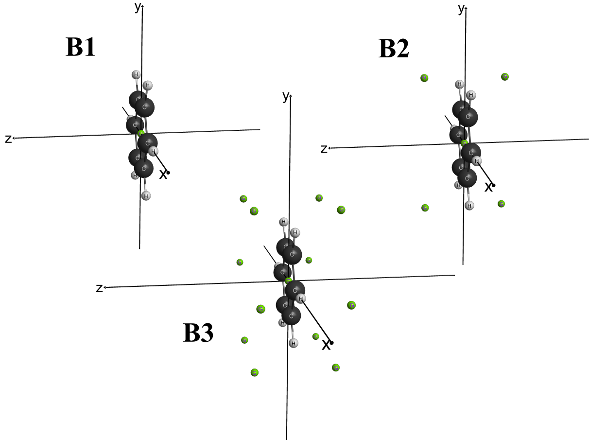
FIG. 2. Illustration of the extra centers (green spheres) in the B1 (one center), B2 (four centers), and B3 (thirteen centers) basis sets, generated with the wxMacMolPlt software [61].
