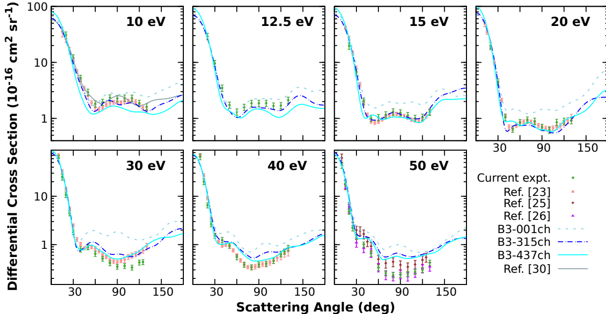
FIG. 4. Elastic differential cross sections for electron scattering from benzene, according to the current and previous measurements (from Cho et al. [23], Sanches et al. [25], and Kato et al. [26]), to the present calculations with the B3 basis set and three multichannel coupling schemes, and to the theoretical results of Barbosa and Bettega [30].
