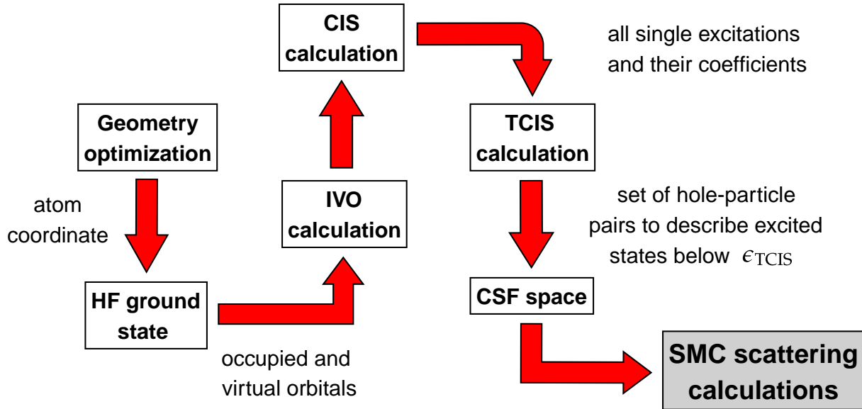
FIG. 1. Scheme illustrating the step-by-step procedure to perform SMC scattering calculations.
