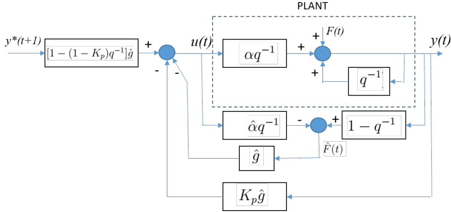
Figure 1: Model Free Control Diagram
