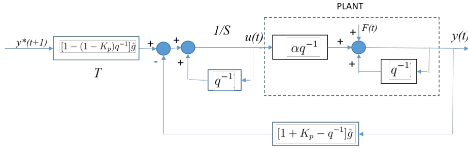
Figure 2: Model Free Control Diagram - R-S-T form.
