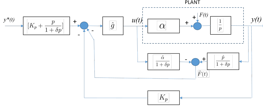
Figure 3: Model Free Control Diagram - Continuous time.
