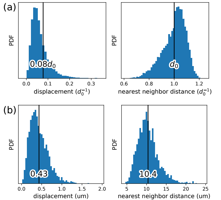
Fig. 4. Distribution of frame-to-frame displacement and nearest neighbor distance in our simulation (a) and in real experimental data (b). Vertical black lines are centered and annotated with the average value of the distributions.
