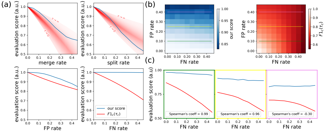
Fig. 5. Our evaluation score responds strongly to simulated merging, splitting and false positive errors and is sensitive to false negatives in scenarios with mixed error types. (a) When a single error type is introduced in simulated data, our score is well correlated with the F1 score except for false negatives, for which it is unresponsive by design. For merge and split conditions, the threshold distance is varied to represent the possible range of F1 score profiles. (b) In mixed FN/FP conditions, our score shows a higher sensitivity to false positives than false negatives, and (c) for high density of false positives, its ranking property can fail. Plots in (c) display the range of values covered by the colored lines in (b).
