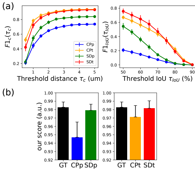
Fig. 7. Our evaluation score can accurately rank three of the four models studied. (a) We use the F1 scores based on centroid detection and on instance segmentation to rank the models using the ground-truth segmentation. We observe better performance from trained models. (b) Our score provides a similar ranking except for the pre-trained model of Stardist3D.
