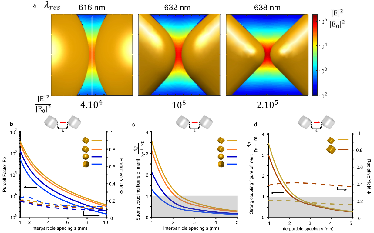
Figure 1: Increased emitter-resonator coupling in gold nanocubes. (a) Simulated local field enhancements, |E/E_0|^2 , in the center of a dimer of 40 nm AuNSs, rounded 30 nm AuNCs or sharp 30 nm AuNCs, with a 2 nm interparticle spacing (the longitudinal resonance wavelengths and the maximum enhancements are provided on the top and bottom of the figures, respectively). (b) Computed Purcell factor F_p (solid lines), and radiative yield \Phi (dashed lines), in dimers of 40 nm AuNSs (blue data), 40 nm rounded icosahedra (light blue), 30 nm rounded AuNCs (orange) and 30 nm sharp NCs (yellow) for a longitudinally coupled emitter positioned in the center and as a function of the interparticle spacing s . (c) Visible strong coupling figure of merit 4g/(\gamma_p + \gamma_0) (solid line, see text for details) as a function of s in the same geometry as (b). (d) Visible strong coupling figure of merit (solid lines) and \Phi (dashed lines) in dimers of 30 nm (yellow) and 40 nm (red) sharp AuNCs for a longitudinally coupled emitter positioned in the center and as a function of the interparticle spacing s .
