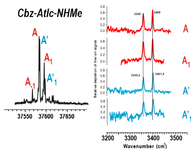
Figure S4.1. Experimental UV spectrum of 2 ( left panel ) and conformer-specific IR/UV spectra obtained by probing the UV transitions A, A 1 and A', A' 1 ( right panel ). The vertical guidelines provide evidence for slight differences between red and blue spectra and hence conformers sharing a same backbone conformation. The UV transition A -1 also give rise to depopulation on the same IR bands as A, showing that they belong to the same conformer. The absolute accuracy of the experimental IR frequency values is \pm 2 cm -1 .
