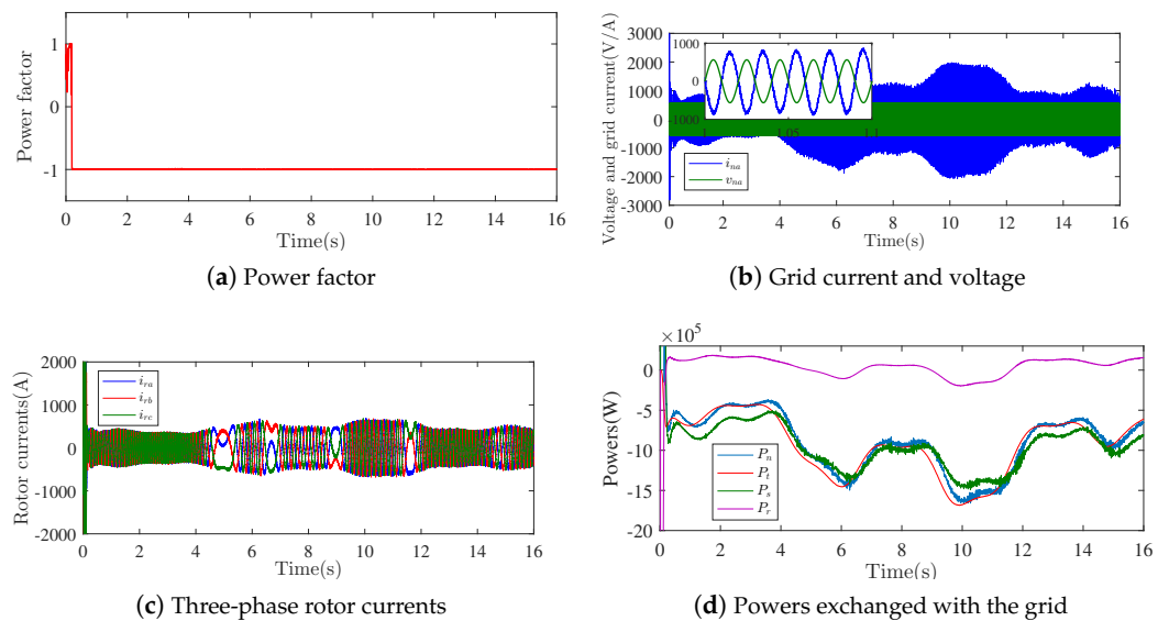
Figure 14. WECS powers.
