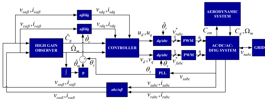
Figure 8. Output feedback control block diagram.
