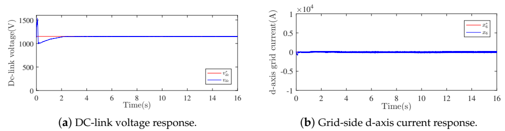
Figure 13. Grid-side results.
