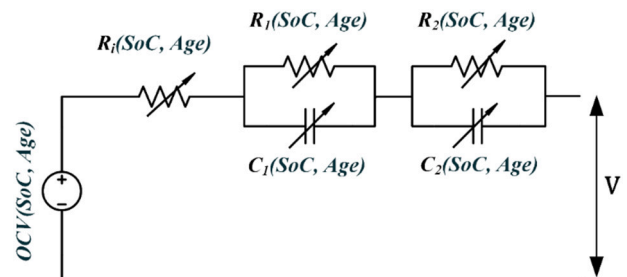
Fig. 11. Proposed second order equivalent circuit model
