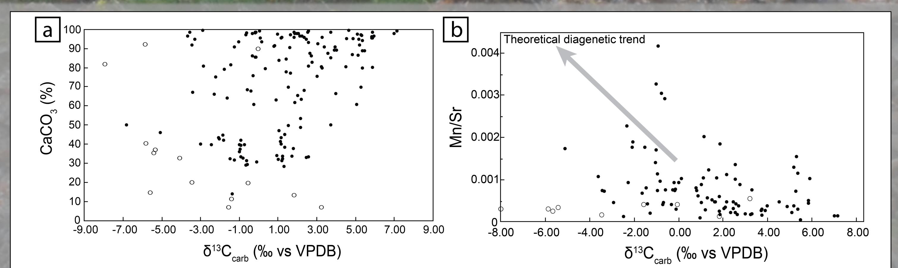
Figure 3 (top): Cross-plots for isotopic and elemental geochemical parameters; a) \delta^{13}C_{carb} vs CaCO_3 content; b) \delta^{13}C_{carb} vs Mn/Sr. \delta^{13}C_{carb} does not follow any diagenetic trend and does not show any correlation.
