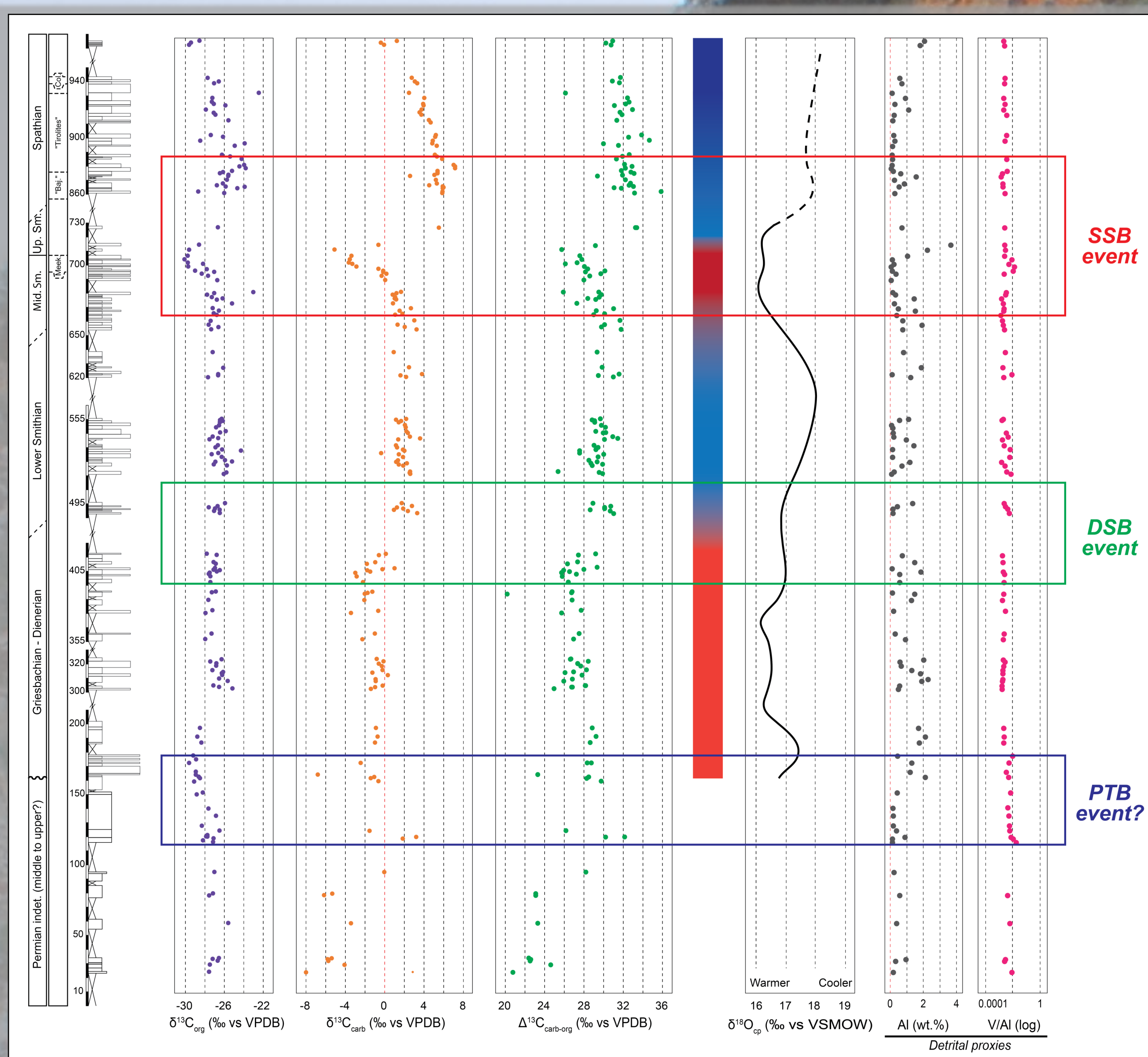
Figure 2: Main geochemical signals in the Hot Springs section with \delta^{13}C_{carb} , \delta^{13}C_{org} , net isotopic effect \Delta^{13}C , and fluctuations of detrital trace and major elements Al and V/Al ratio. \delta^{18}O_{org} and paleotemperatures trends from Romano et al. (2013). Ammonoid biozones: Meek., Meekoceras; "Baj.", Bajarunia; Col., Columbites.
