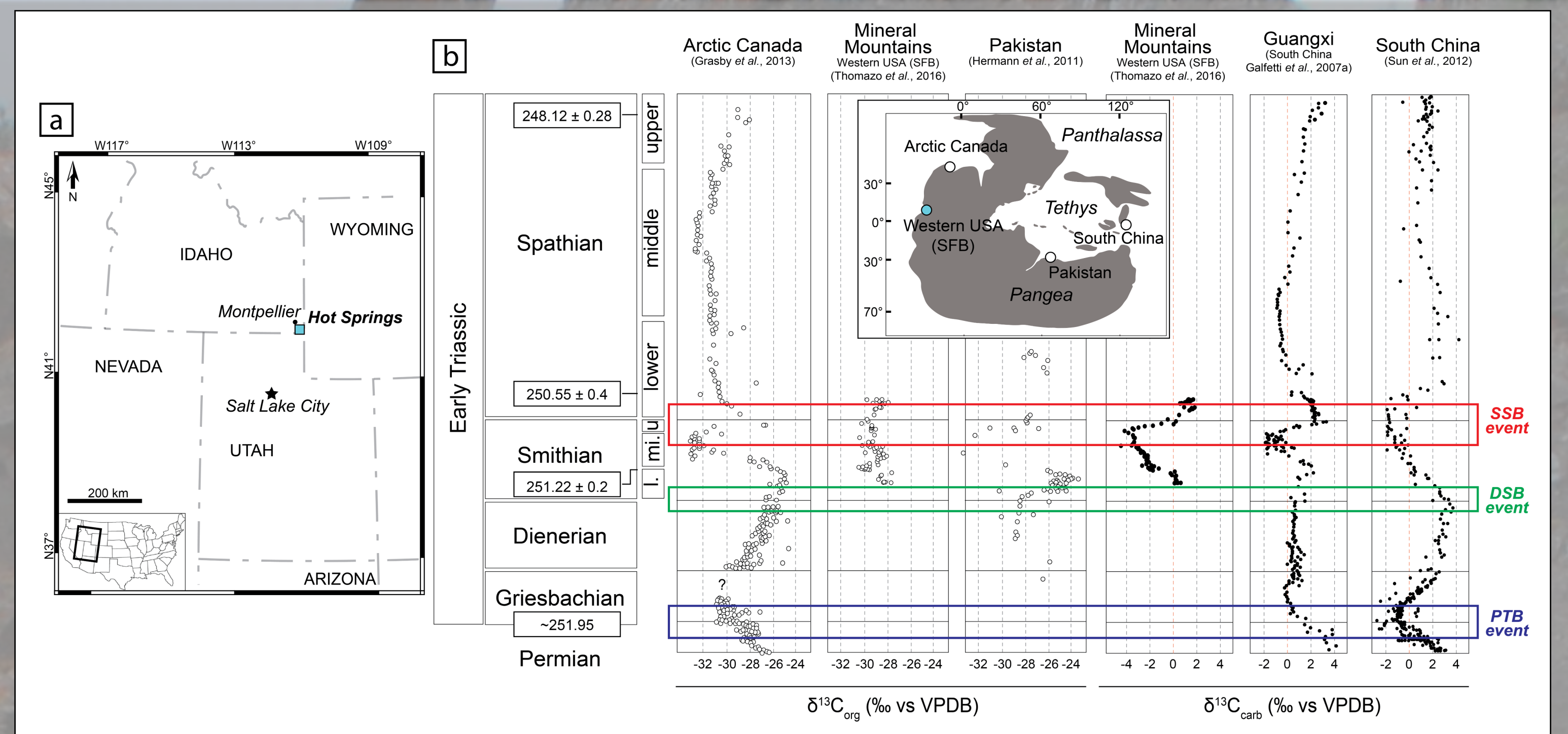
Figure 1: a) Map of the studied area and location of the Hot Springs section; b) Worldwide Early Triassic variations of the \delta^{13}C signal for both carbonate and OM reservoirs.
