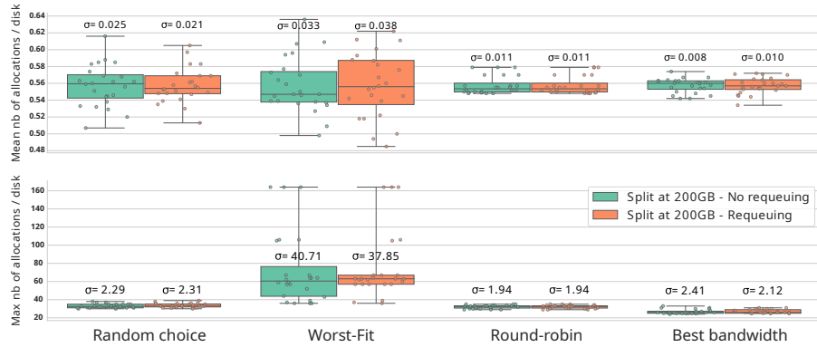
Fig. 6. Mean (top) and max (bottom) number of allocations per disk, grouped by algorithms, for 32TB platform and split strategy. Storage layout 1N1D excluded. Dots plot the mean and max number of allocations of each disk separately.
