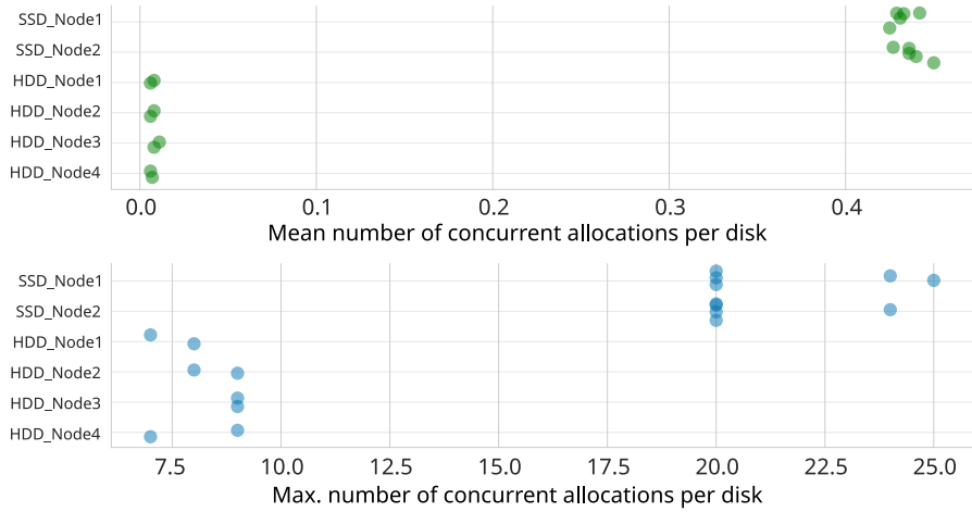
Fig. 8. Mean and maximum number of allocations per disks, grouped by node, when using a 32TB heterogeneous platform composed of nodes using either SSDs or HDDs.
