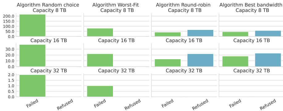
Fig. 7. Maximum number of failed and refused split requests, grouped by algorithm and platform capacity: 8, 16 and 32TB (no failed or refused requests at 64TB).
