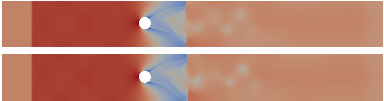
FIGURE 13. Barotropic flow past a cylinder - density at time t = 1 . Top: upwind scheme. Bottom: centered limited scheme.
