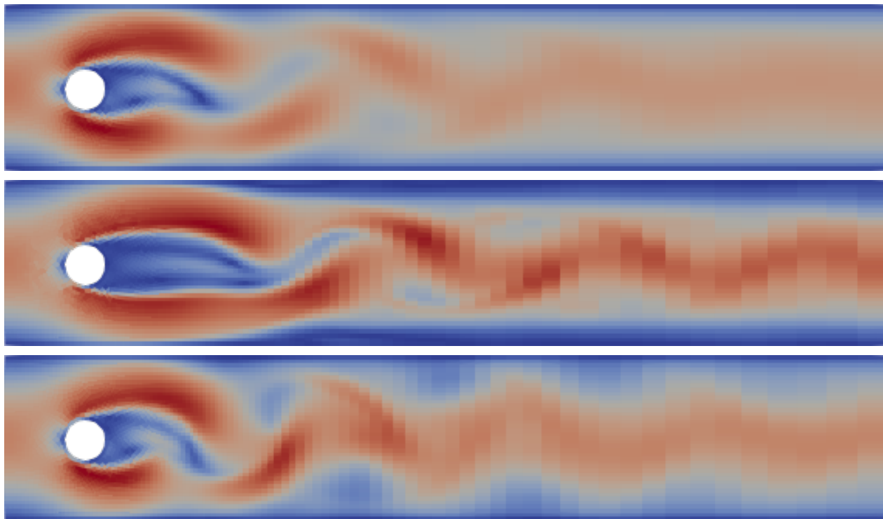
FIGURE 4. Incompressible flow past a cylinder - Magnitude of the velocity at time t = 5 (coarse mesh). From top to bottom: upwind scheme, centered scheme, centered limited scheme.
