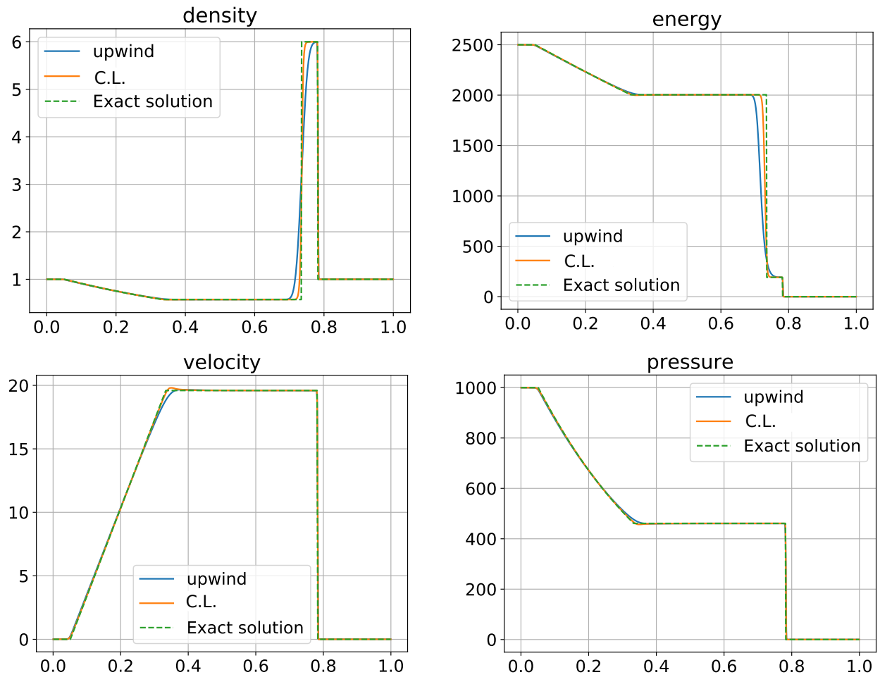
FIGURE 15. Riemann problem for the Euler equations - Comparison of the results of the Test case 3 of [34] obtained with the two following schemes. Orange: MUSCL discretization, for the scalar variables, and centered limited (C.L.), for the velocity, of the convection terms. Blue: first-order upwind discretization of the convection terms. Exact solution is plotted in green.
