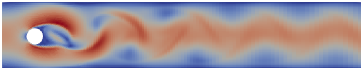
FIGURE 5. Incompressible flow past a cylinder - Magnitude of the velocity at time t = 5 for the most refined mesh, with the centered scheme.
