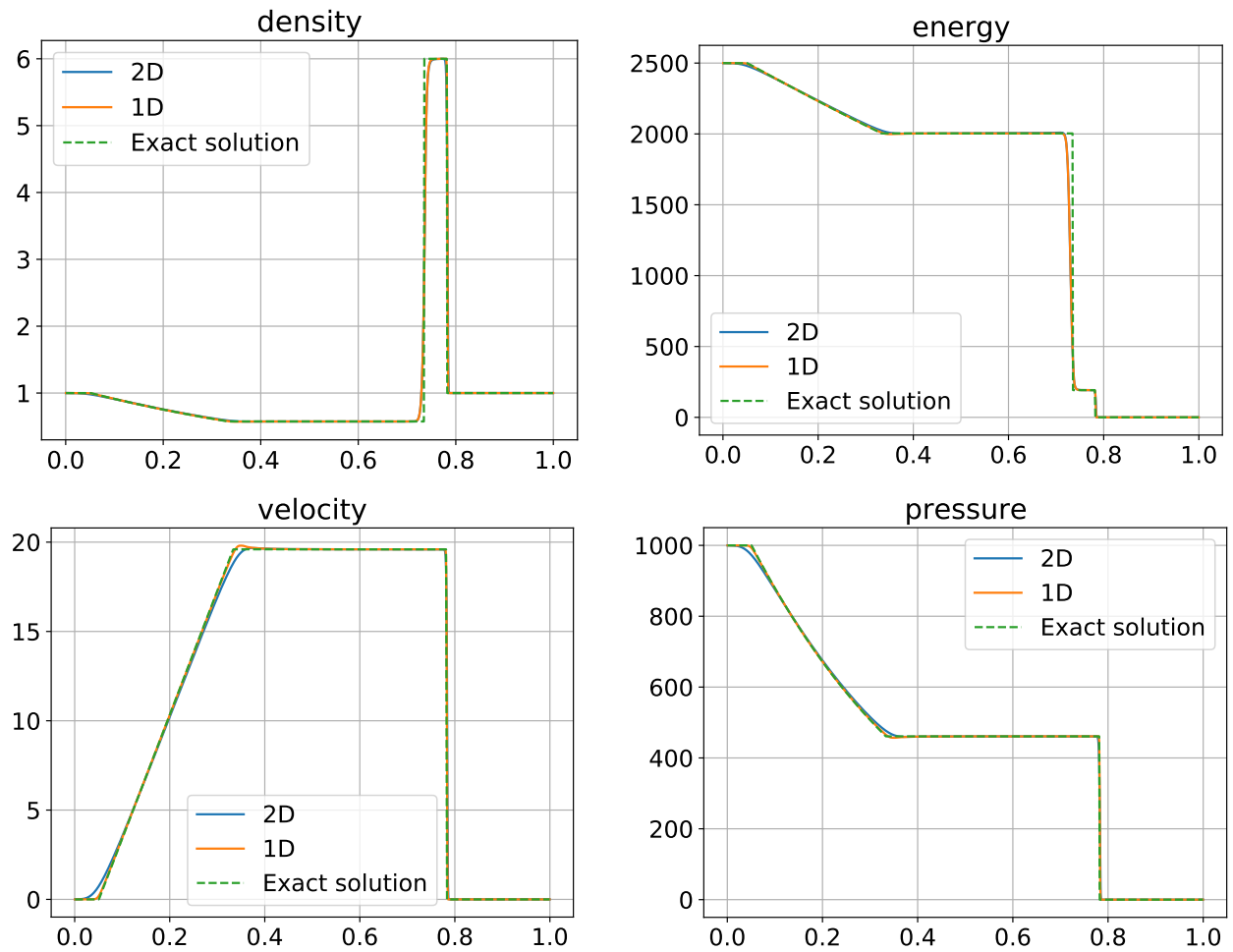
FIGURE 16. Riemann problem for the Euler equations - Comparison of the results of the Test case 3 of [34] obtained with a MUSCL discretization of the scalar variables convection terms and the centered limited discretization of the velocity convection term, on a one dimensional domain (in orange) or a fictitious two dimensional domain (in blue). Exact solution is plotted in green.
