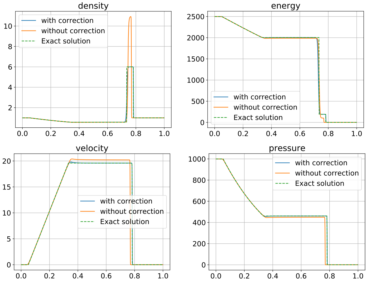
FIGURE 14. Riemann problem for the Euler equations - Comparison of the results of the Test case 3 of [34] for a MUSCL discretization of the scalar variables convection terms and the centered limited discretization of the velocity convection term, with the corrective term of Section 4.3 (in blue) or without it (in orange). Exact solution is plotted in green.
