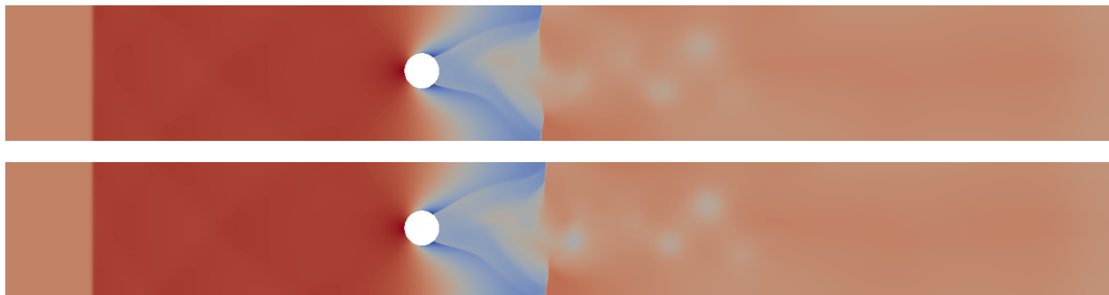
FIGURE 13. Barotropic flow past a cylinder - density at time t = 1 . Top: upwind scheme. Bottom: centered limited scheme.
