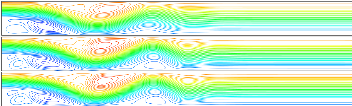
FIGURE 10. Backward-facing step - Streamlines at time t = 20 . From top to bottom: upwind, centered, and centered limited schemes.
