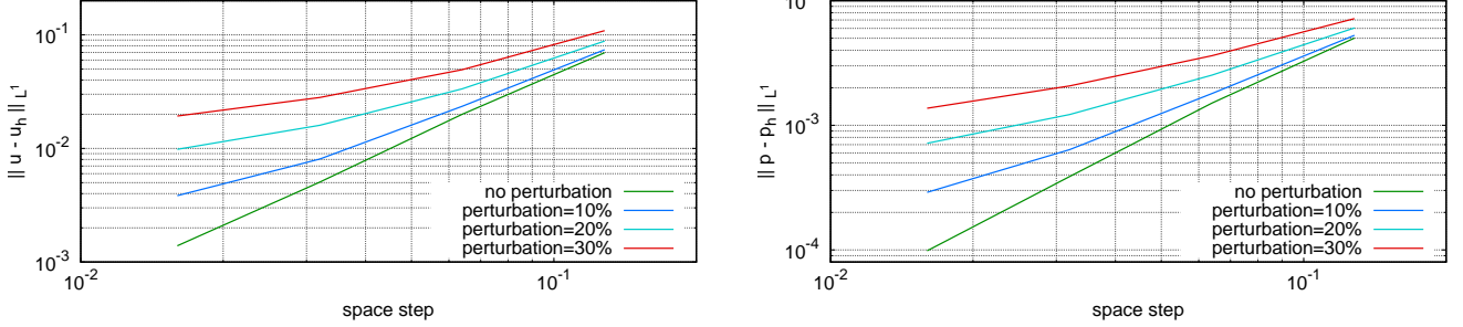
FIGURE 12. Barotropic travelling vortex - L^1 norm of the error obtained at the final time with the centered limited scheme for the velocity (left) and the pressure (right), with unstructured meshes generated by a random perturbation of the vertices location.
