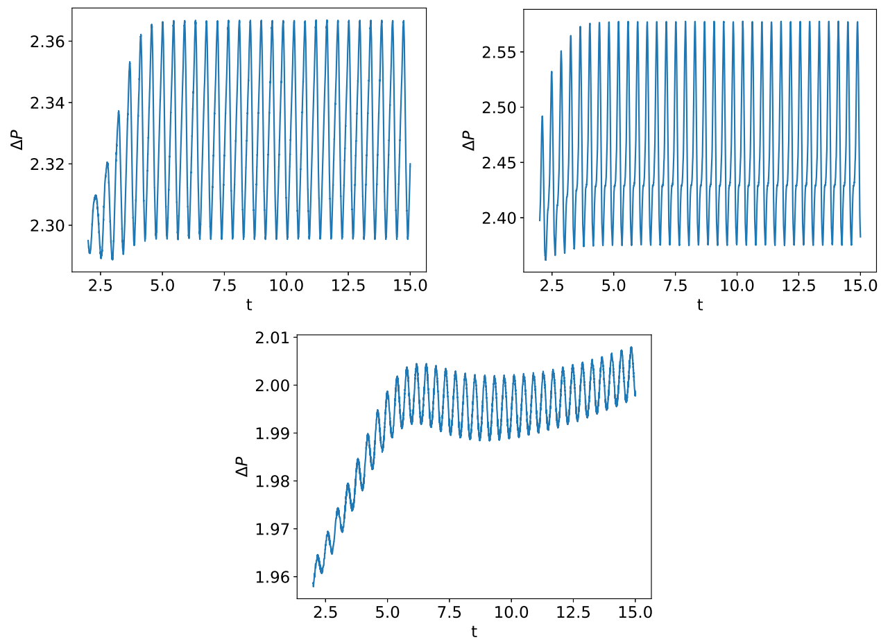
FIGURE 7. Incompressible flow past a cylinder - \Delta P as a function of time on the coarsest mesh. Top-left: upwind scheme. Top-right: centered limited scheme. Bottom: centered scheme.
