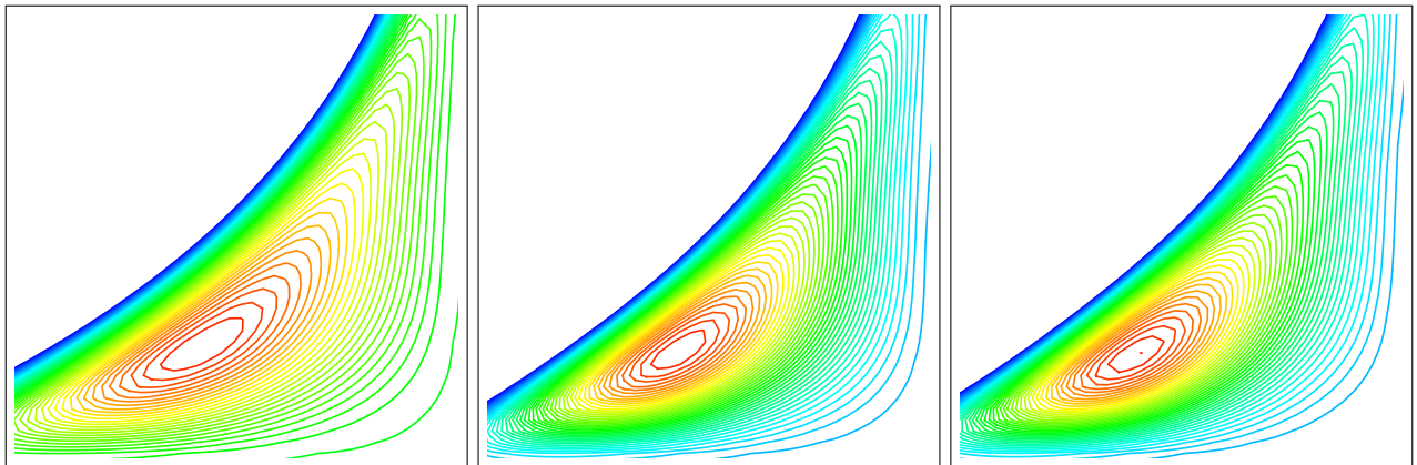
FIGURE 9. Lid-driven cavity - Secondary vortex. From left to right: results with the upwind, centered, and centered limited scheme.
