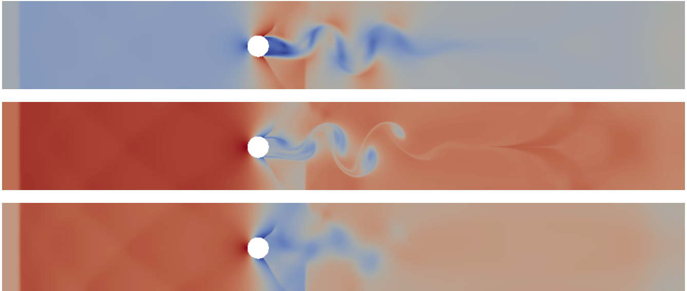
FIGURE 17. Flow past a cylinder, Euler equations - From top to bottom, velocity, density and pressure at time t = 1 .
