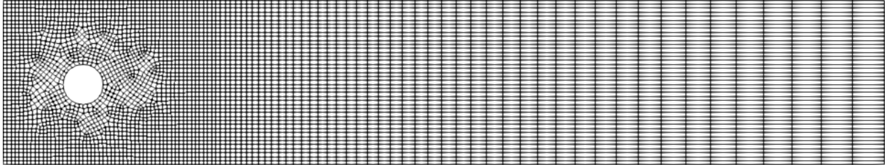
FIGURE 3. Incompressible flow past a cylinder - Coarse mesh.
