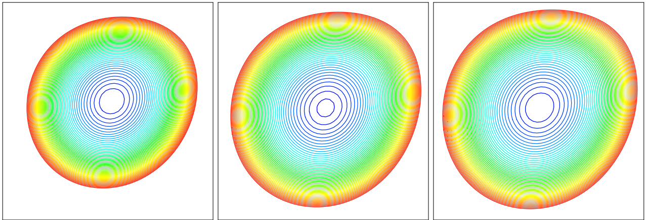
FIGURE 8. Lid-driven cavity - Primary vortex. From left to right: results with the upwind, centered, and centered limited scheme.
