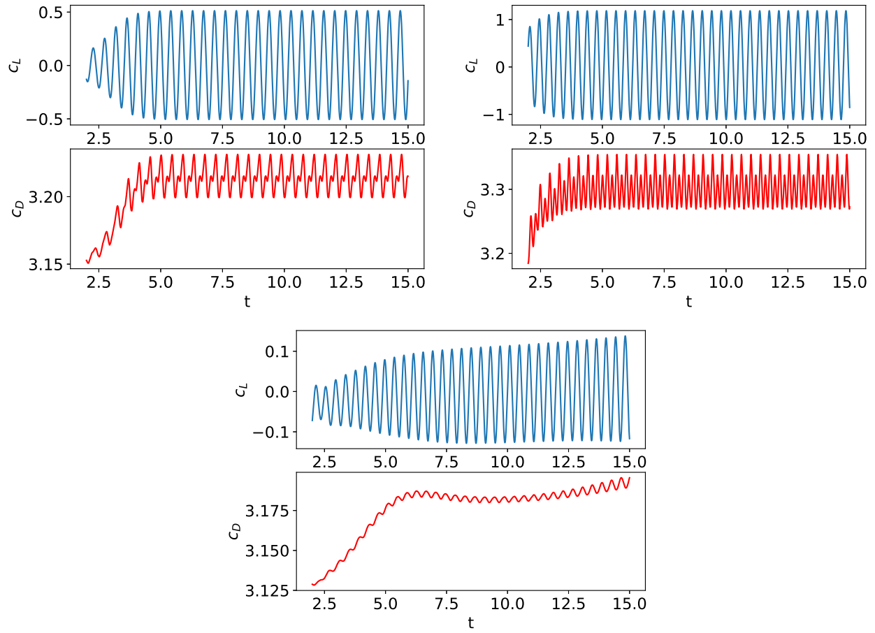
FIGURE 6. Incompressible flow past a cylinder - Drag and lift coefficient as a function of time (coarse mesh). Top-left: upwind scheme. Top-right: centered limited scheme. Bottom: centered scheme.
