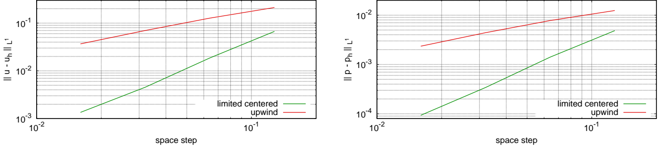
FIGURE 11. Barotropic travelling vortex - L^1(\Omega) norm of the error obtained at the final time with the centered limited scheme and a first-order scheme, for the velocity (left) and the pressure (right). Here the mesh size is computed as h = 3.2/n , for a n \times n mesh (so \text{diam}(K) = \sqrt{2}h , for K \in \mathcal{M} ).
