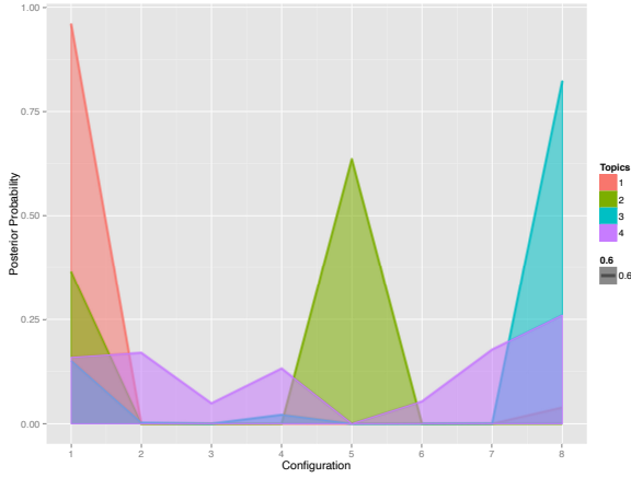
Fig. 4: Distribution of configurations, featuring \Lambda^{(k)} for each of the 4 topics.
