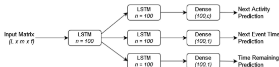
Fig. 1. Model architecture: L : number of sentences, m : maximum trace length, f : number of features, n : number of neurons, c : number of unique
