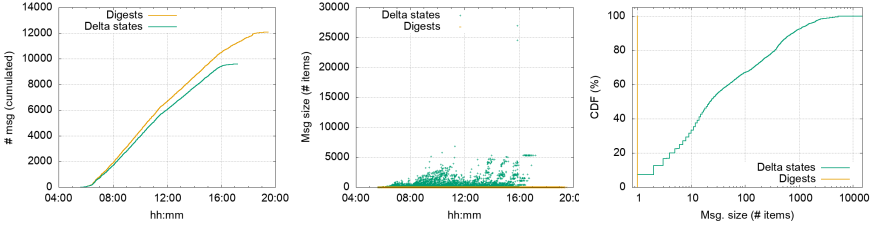
(Δ-SB-a) Evolution of the number of messages exchanged by neighbor nodes (cumulated)
