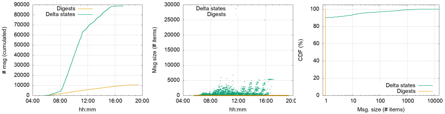
(Δ-SBT-a) Evolution of the number of messages exchanged by neighbors nodes (cumulated)
