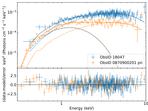
Fig. 4. Spectra of Chandra ObsID 18047 (blue) and XMM-Newton /pn ObsID 0870900201 (orange), representative of the HHL and SLL states, respectively. Spectra are fitted with the model \text{tbabs} * \text{tbabs} * (\text{diskbb} + \text{diskbb}) (solid line) with the two black-body components plotted as dashed lines. Bottom panel : residuals of the fit.
