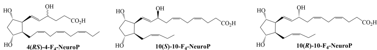
Figure 3. Representation of chemical structures of 4- and 10-F 4 t-NeuroP isomers.
