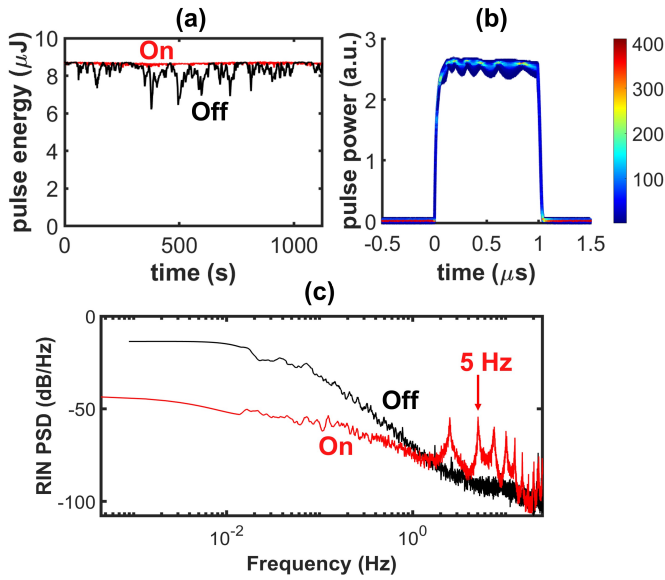
Fig. 4. a) Combined pulse energy evolution with (red) and without (black) active phase control during 1000 s of operation at 6.9 A measured by PhD1. b) Density plot of \sim 500 sets of combined pulses during 1000 s measured by PhD2. c) Relative intensity noise PSD of the stabilized (red) and free-running (black) power measurements (PhD1).
