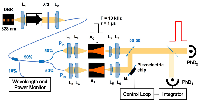
Fig. 1. Diode-laser-based source with coherent beam combination of two high brightness tapered amplifiers ( A_1 and A_2 ).
