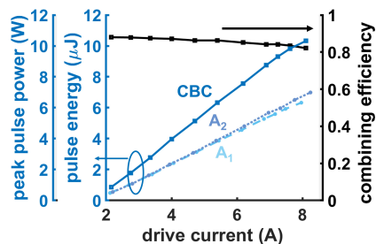
Fig. 5. Measured individual and combined pulse energies and combining efficiencies at drive currents from 2.2 A to 8.1 A.
