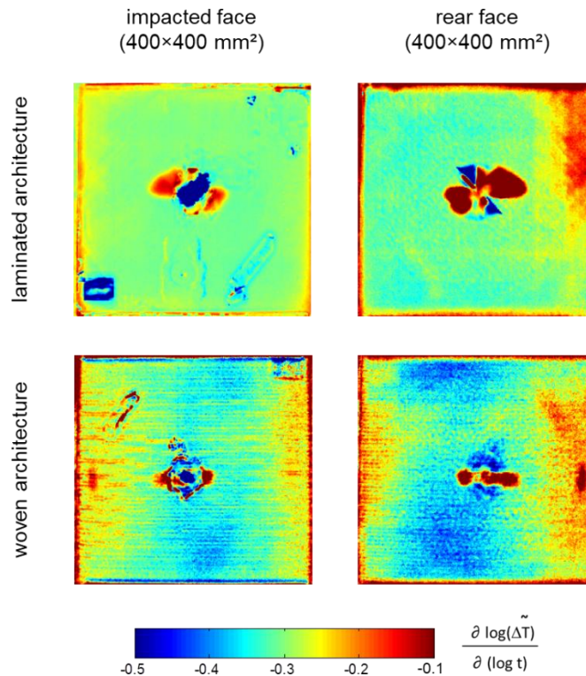
Fig. 2. Comparison between the damage patterns of 2.4mm-thick laminate (top) and woven (bottom) carbon/epoxy composite coupons, submitted to the same electric arc. First logarithmic derivative fitted temperature variation for both impacted (left) and rear (right) faces of the coupons.
