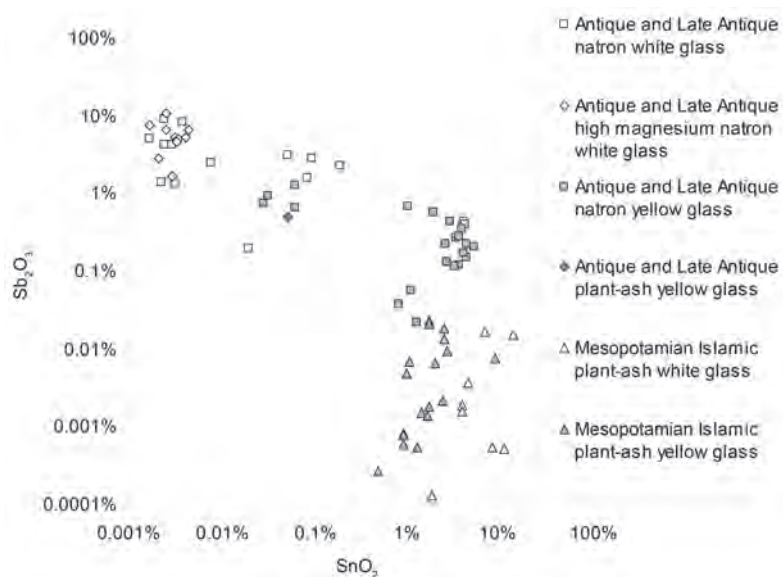
Fig. 8 Concentrations of \text{SnO}_2 vs \text{Sb}_2\text{O}_3 for the different white and yellow glasses analysed from Ribe. The natron Antique and late Antique glasses are clearly distinguished from the Islamic soda plant ash glasses by their opacifiers. While antimony and tin are both used either alone or mixed in natron Antique and late Antique glasses, only tin is used in Islamic soda plant ash glasses. – (Diagram CNRS/IRAMAT-CEB)
