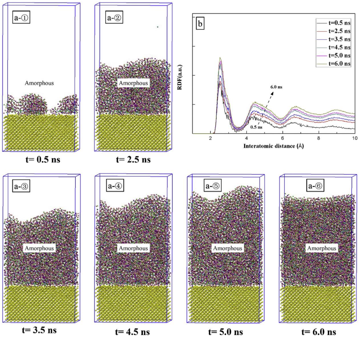
Figure 28. Snapshots and RDF of \text{Al}_2\text{Co}_9\text{Cr}_{32}\text{Cu}_{39}\text{Fe}_{12}\text{Ni}_6 deposited on Si (100) substrate at different times t . ● Al, ● Co, ● Cr, ● Cu, ● Fe, ● Ni, ● Si. Reprinted from Ref. 295
