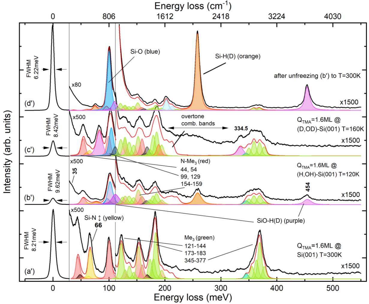
Figure 5. HREELS spectra (black curve) and peak-deconvolution after background subtraction (red line) of (a) clean Si(100)-2×1 at 300 K and (a') exposed to Q_{\text{TMA}}=1.6 ML at 300 K, (b) (H,OH)-Si(100) at 120 K and (b') exposed to Q_{\text{TMA}}=1.6 ML at 120 K, (c) (D,OD)-Si(001) at 160 K, (c') exposed to Q_{\text{TMA}}=1.6 ML at 160K and (d') shows (b') after unfreezing to T=300 K. Peak positions in the figure are given in meV. “Me” is for CH 3 . Color code: Si phonons (grey), SiO-H/SiO-D (purple), Si-H/Si-D (orange), Si-O (blue), Si-N (yellow), N-Me 3 (red), Me 3 (light/dark green) and non-attributed (black).
