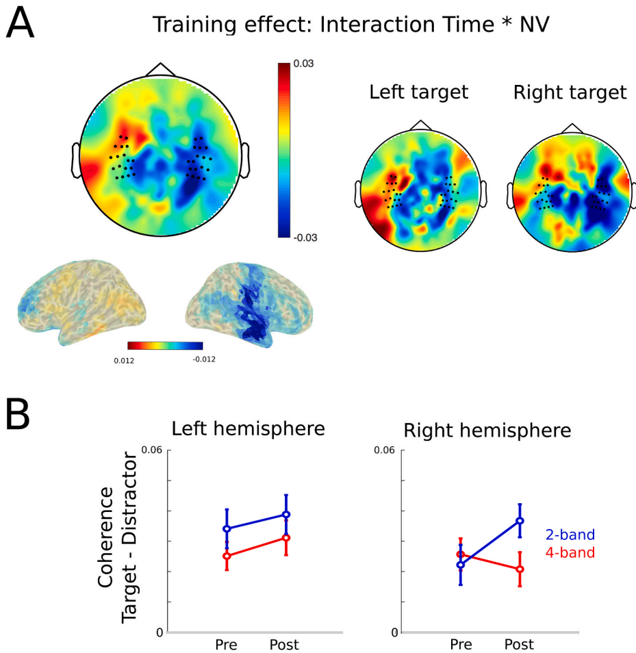
Fig. 8. Contrast between tracking of target speech and of distracting speech in the delta range (A) Topographies and source reconstruction of interaction between factors time and NV ( Coh_{Post} - Coh_{Pre} ) 4band} - (Coh_{Post} - Coh_{Pre})_{2band}. A significant interaction time*NV*hemisphere was observed. Training significantly impacted the contrast between target and distractor speech in the right hemisphere: distracting and target speech-brain coherence is less distinguishable in this hemisphere after training for the 4 band-NV condition. This effect was not dependent on the side of target position. (B) Delta tracking of the contrast between target and distracting speech averaged across selected channels in each hemisphere, when in competition with distracting 4-band NV speech (red) or 2-band NV speech (blue). Error bars indicated standard error of the mean. (For interpretation of the references to colour in this figure legend, the reader is referred to the Web version of this article.)
