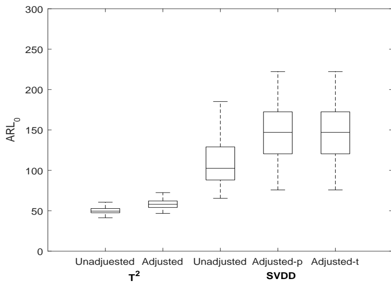
(b) F_{SAT}(T, X|4, 2.5, 100, 0.1, 0.5)
