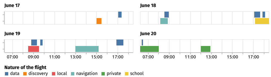
Figure 3. Comparison of detected activity based on Mode A/C data with flight logs for a private aircraft based at Eyguières airfield LFNE nearby our LFM receiver. In spite of no ADS-B-compliant equipment, it is possible to detect a local activity of the aircraft.
