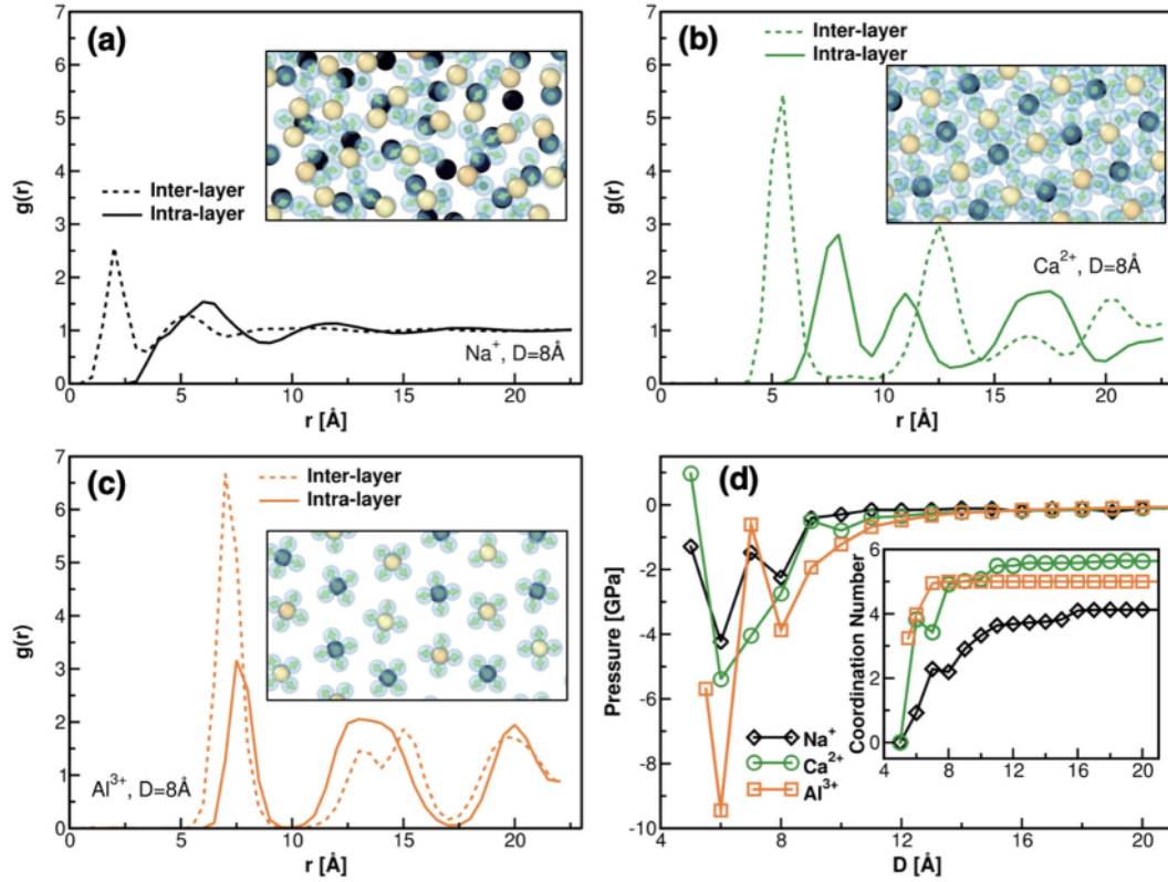
Figure 6. Interlayer and intralayer correlations at \sigma = 3e^-/\text{nm}^2 and D = 8 Å for (a) sodium, (b) calcium, and (c) aluminum. Reducing the pore size to D = 8 Å leads to higher peaks in g(r) when compared to Figure 5c; the interlayer correlations especially increase. This is also reflected and visualized in the corresponding simulation snapshots. (d) The growth of interlayer correlations gives rise to a greater attraction between the surfaces. Nevertheless, the stability of the hemispherical hydration shells still has an effect; the few spikes in the pressure are rooted in changes in the coordination number, or size, of the n -mers (inset).
