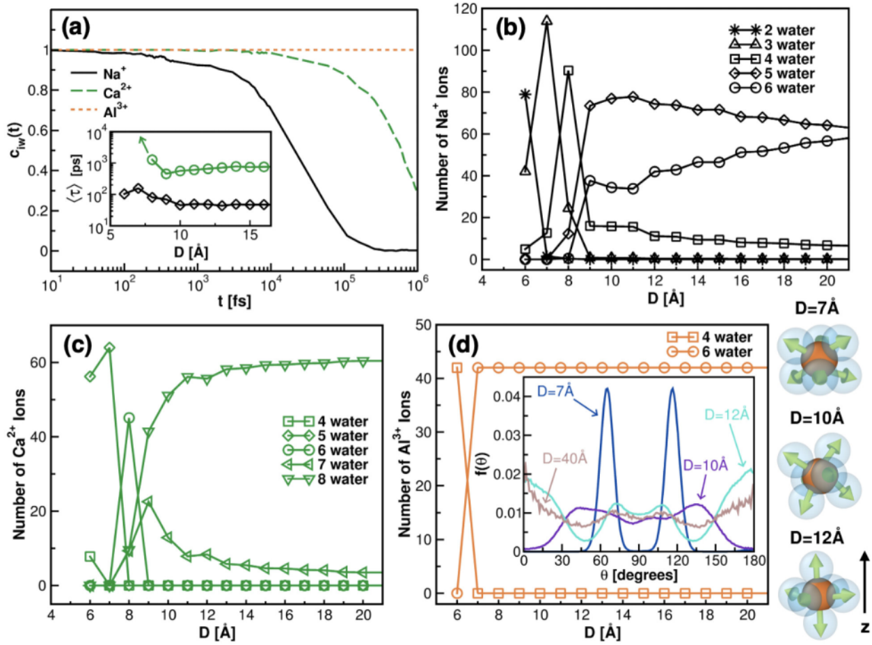
Figure 3. (a) Time correlation of ion–water bonds at D = 20 Å and the relaxation time for Na + –water and Ca 2+ –water bonds at various values of D . Water initially bound to Al 3+ ions remains bound indefinitely, and the relaxation time for Na + –water bonds is generally an order of magnitude less than that for Ca 2+ –water bonds, implying that sodium hydration shells are the least persistent. However, where the Na + pressure is at its minimum, D = 7 Å, the sodium n -mers are considerably more enduring. Plots (b) and (c) reveal that sodium and calcium have full hydration shells of 5 to 6 and 7 to 8 water molecules, respectively, at large separations. When the confinement is increased, there are key values of the pore size in which the size of the shells notably changes, corresponding to dips and spikes in the pressure. Aluminum hydration shells, being the most persistent, are able to endure at lower separations by exerting a stronger push against the confining wells; the persistence of these n -mers is why the pressure becomes less attractive at higher valency for \sigma = 1e^-/\text{nm}^2 . Even so, the distribution of the bond angles, or the shape of the Al 3+ 6-mers, does change significantly (see (d)) and is also correlated with fluctuations in the pressure.
