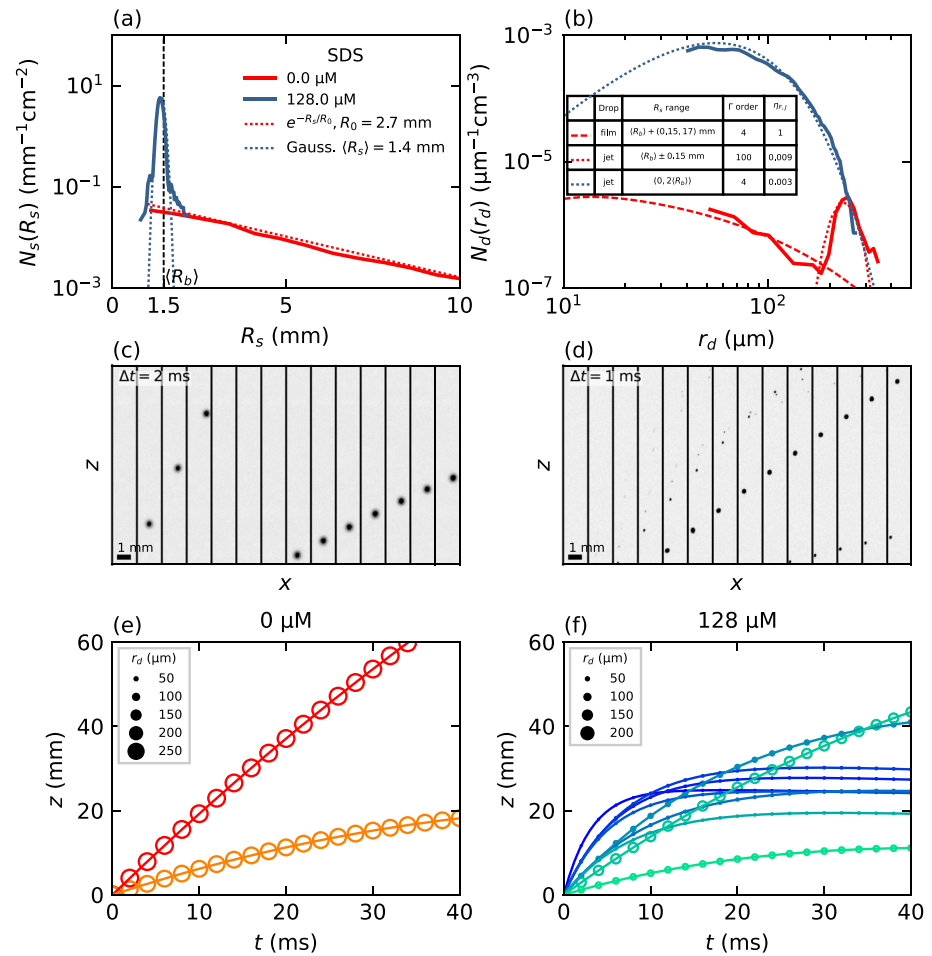
Figure 4. (a) Surface bubble radius N_s(R_s) and (b) drop radius N_d(r_d) distributions in deionized water (red lines) and contaminated water sodium dodecyl sulfate (SDS), c = 128 \mu\text{M} , blue lines, for bulk bubbles with mean radius \langle R_b \rangle = 1.5 mm. (a) Measured distributions are fitted by integrable functions (dotted lines). (b) Dashed and dotted lines are the integration by (1) of the corresponding surface bubble distributions, considering respectively a film drop or a jet drop mechanism. Integration parameters are given in the legend. (c and d) Image sequences highlighting the bursting of a single bubble (located below the frame), in (c) clean water (2 drops) and (d) with SDS at c = 128 \mu\text{M} (9 drops). Acquisition rates are respectively 500 and 1,000 Hz, scale bar is 1 mm wide. (e and f) Drop vertical trajectory z(t) for the 2 bubble bursting shown in (c) and (d): (e) clean water (2 drops) and (f) with SDS at c = 128 \mu\text{M} (9 drops). Color indicates the drop ejection number (from darker colors for the first ejected drop to lighter color to the subsequent ones) and size of the symbols indicates the size of the drop.
