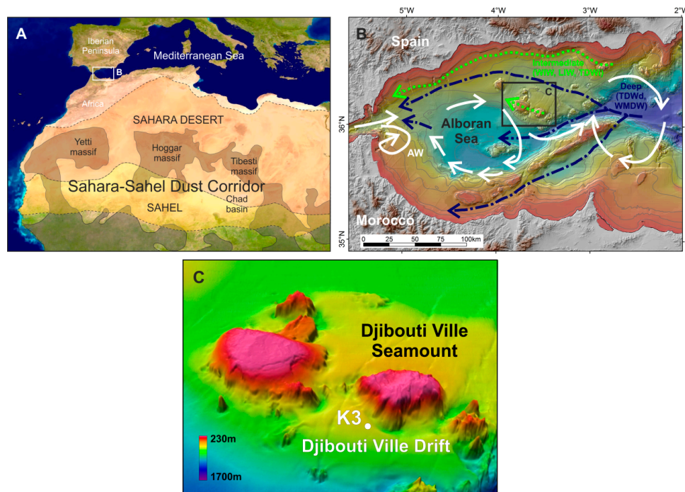
Figure 1. (A) Local setting of the study area in the Western Mediterranean Sea and the Sahara–Sahel Dust Corridor. The outcrop of basement rocks is based on [19]. (B) Main trajectories of the water masses circulation in the Alboran Sea (based on [18]). Legend: AW, Atlantic Water; WIW, Western Intermediate Water; LIW, Levantine Intermediate Water; TDW, Tyrrhenian Dense Water (i: intermediate, d: deep); WMDW, Western Mediterranean Deep Water. (C) 3D bathymetric view of the Djibouti Ville Seamount showing the location of the K3 sediment core at the Djibouti Ville drift.
