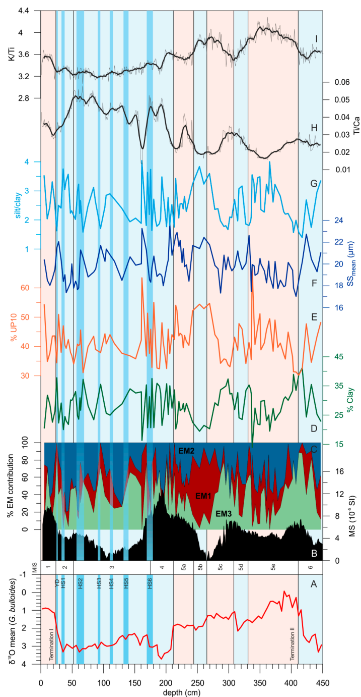
Figure 6. Vertical variation in the grain-size and geochemical parameters in core K3. (A) Chronostratigraphic framework based on \delta^{18}\text{O} of Globigerina bulloides (plotted with reverse Y axis) (see Figure 3 for more details). (B) Magnetic susceptibility ( \text{MS } 10^{-5} \text{ SI} ). (C) End-member scores (%contribution) displaying the proportion of variance explained by the 3 end-members for each individual sample. (D) Clay content (vol.%). (E) UP10 fraction (vol.%) that corresponds to particles >10 \mu\text{m} [13,14]. (F) Mean grain-size of the sortable silt fraction ( \text{SS}_{\text{mean}} ) corresponding to the 10–63 \mu\text{m} particle size range [3]. (G) silt/clay ratio. (H) Ti/Ca ratio of XRF counts. (I) K/Ti ratio of XRF counts. Marine Isotope Stages (MIS) of the stadials (MIS 6, 5d, 5b, 4, 3, and 2) are indicated in clear blue and the interstadials (MIS 5e, 5c, 5a, and 1) are in light orange [30]. The Heinrich Stadials (HS 6 to 1, [57]) and Younger Dryas (YD, [20]) are indicated in dark blue.
