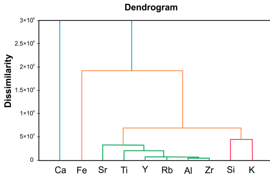
Figure 7. Dendrogram from the Hierarchical Cluster Analysis (HCA) by using the single linkage as agglomeration method of the Euclidean distances.
