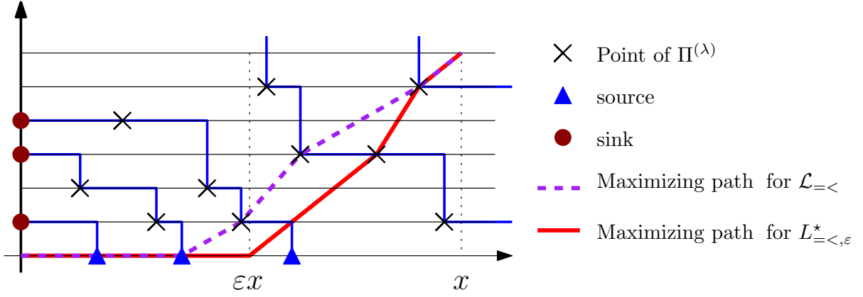
Figure 4: A sample of \Pi_{x,t}^{(\lambda)} , sources, sinks, and the corresponding trajectories of particles (in blue). Here \mathcal{L}_{=<}(\Pi_{x,t}^{(\lambda)} \cup \text{So}_x^{(\bar{\alpha})} \cup \text{Si}_t^{(\bar{p})}) = 5 (pink path) and L_{<}^{(\alpha,p)}(t) = 2 (two remaining particles at the top of the box).
