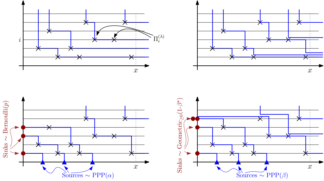
Figure 3: Our four variants of the Hammersley process (time goes from bottom to top, trajectories of particles are indicated in blue). Top left: The process L_{<}(t) . Top right: The process L_{\leq}(t) . Bottom left: The process L_{<}^{(\alpha, p)}(t) . Bottom right: The process L_{\leq}^{(\beta, \beta^*)}(t) .
