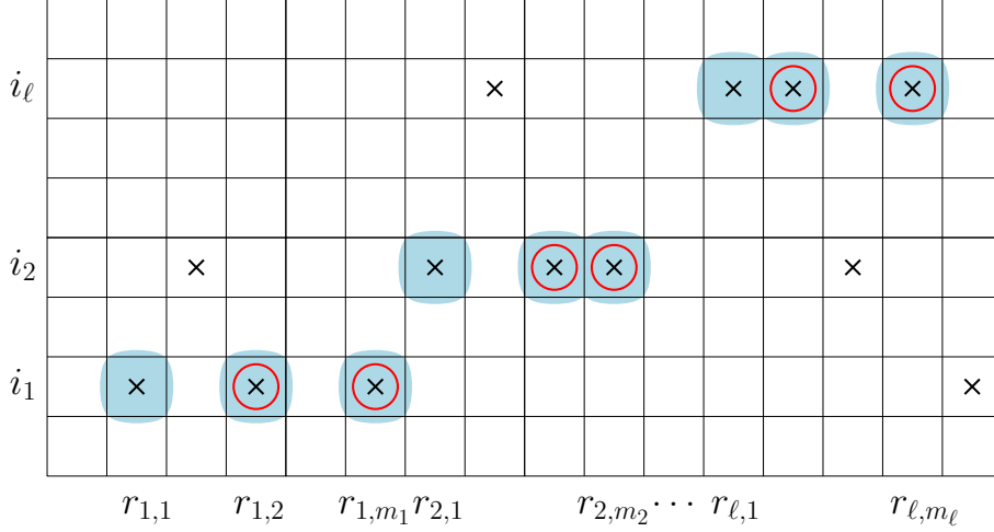
Figure 2: The event F . (Ties are surrounded in red. Points with blue background represent the subsequence with \delta\sqrt{n} ties.)
