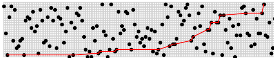
Figure 1: A uniform 5-multiset permutation S_{5,30} of size n = 30 and one of its longest non-decreasing subsequences.
