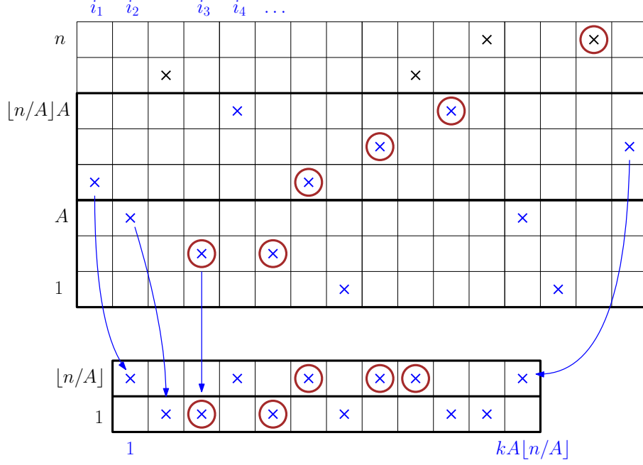
Figure 4: Illustration of the notation of Lemma 14. Top: the multiset permutation S_{k;n} . Bottom: the corresponding \tilde{S} . The longest non-decreasing subsequence in S_{k;n} (circled points) is mapped onto a non-decreasing subsequence in \tilde{S} , except one point with height > A\lfloor n/A \rfloor .
