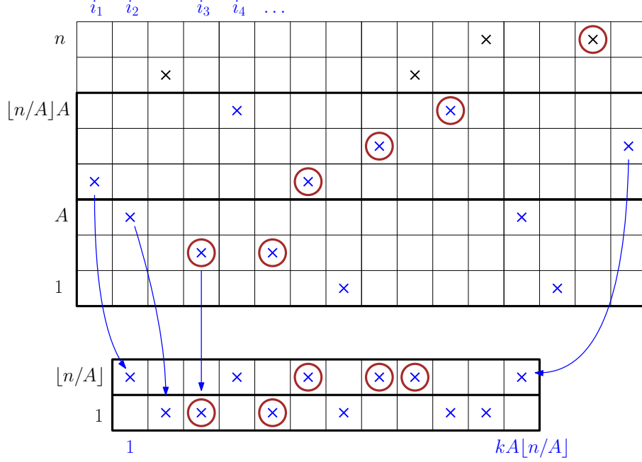
Figure 4: Illustration of the notation of Lemma 13. Top: the multiset permutation S_{k;n} . Bottom: the corresponding \tilde{S} . The longest non-decreasing subsequence in S_{k;n} (circled points) is mapped onto a non-decreasing subsequence in \tilde{S} , except one point with height > A\lfloor n/A \rfloor .
