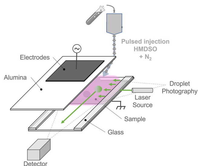
FIGURE 1 Schematic view of the experimental setup coupling pulsed hexamethyldisiloxane (HMDSO) aerosols with dielectric barrier discharges for thin film deposition. The laser source and detector used for droplet scattering measurements are also shown.
