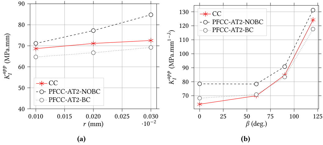
Figure 9: Apparent (a) stress intensity factor variation as a function of the hole radius and (b) generalized stress intensity factor variation as a function of the V-notch angle obtained using either the CC or the LF-PF model with or without Dirichlet damage boundary condition for 3YSZ ceramic.
