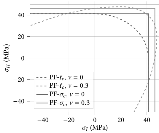
Figure 2: Homogeneous solution failure surface in the space of principal stresses obtained for E = 3 GPa, \mathcal{G}_c = 300 J/m 2 , \nu = 0 or \nu = 0.3 , using either AT1 implementation ( \ell_c = 0.2 mm) or the proposed strength-based PF formulation ( \sigma_c = 41 MPa for \nu = 0 and \sigma_c = 46 MPa for \nu = 0.3 ).
