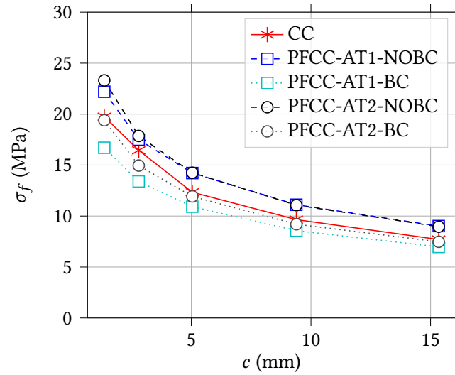
Figure 7: Failure stress variation as a function of the square hole side obtained using either the CC, the AT1 or the AT2 version of the LF-PF model considering or not Dirichlet damage boundary condition on the V-notch tip.
