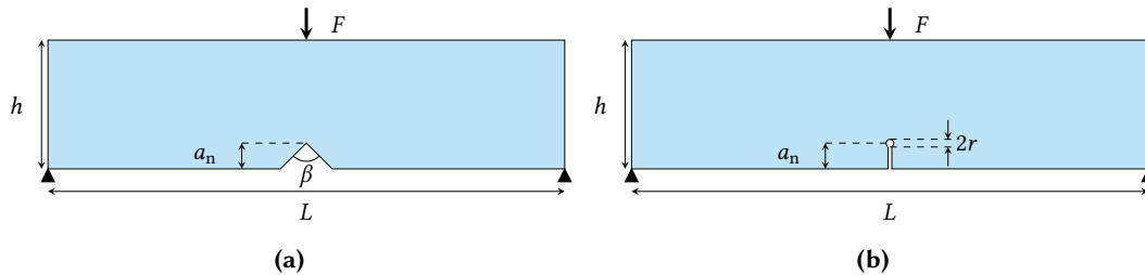
Figure 8: Abaza's benchmark geometries under investigation: (a) three-point bending specimen containing a V-notch and (b) three point bending specimen containing a crack blunted by a hole.
