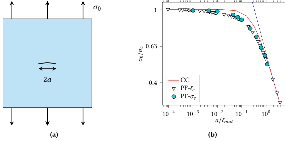
Figure 3: (a) Infinite media containing a crack of length 2a subjected to a remote stress \sigma_0 and (b) variation of the critical stress at crack propagation normalized by the material tensile strength as a function of the initial crack length normalized by the material characteristic length obtained using either the CC, the classical PF or the LF-PF model. The blue dashed line indicates Griffith's solution.
