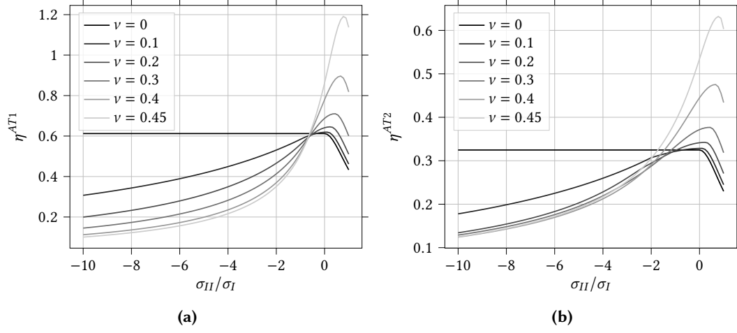
Figure 1: Variation of the normalized tensile strength \eta as a function of the principal stress ratio \sigma_{II}/\sigma_I obtained for a) AT1 and b) AT2 implementation of the classical PF approach.
