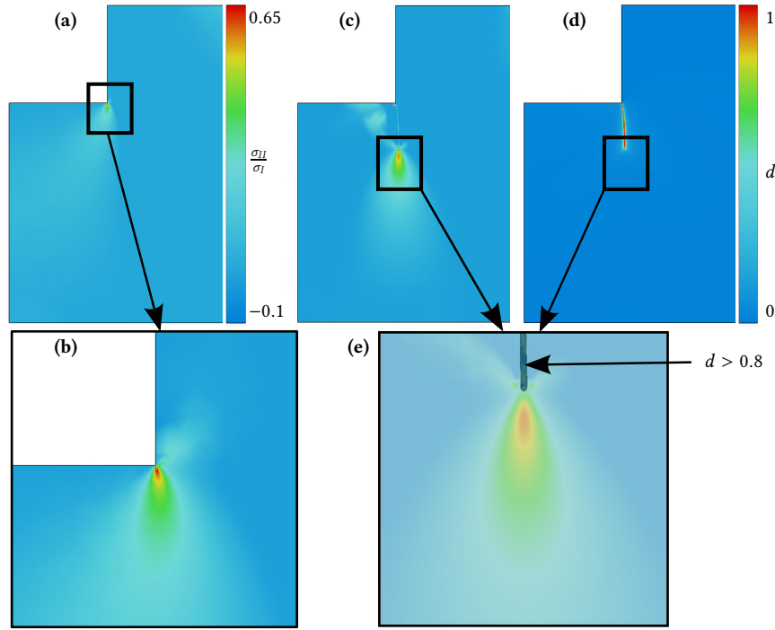
Figure 5: Principal stress ratio \sigma_{II}/\sigma_I distribution around the square hole corner (a-b) before crack initiation and (c,e) after crack propagation on a certain distance and (d) corresponding damage distribution (the superimposed black zone in (e) corresponds to an area where damage is larger than 0.8. A d = 1 Dirichlet boundary condition is prescribed on the V-notch tip node in this example.
