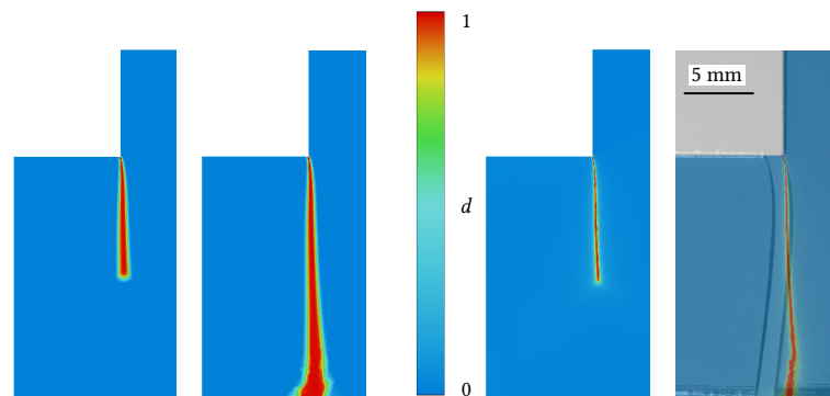
Figure 6: Damage distribution around the square hole in the specimen obtained using (left) AT1 or (right) AT2 versions of the LF-PF model. The final crack path obtained with AT2 version is compared to an experimental observation of the specimen after failure (Doitrand et al. 2021).
