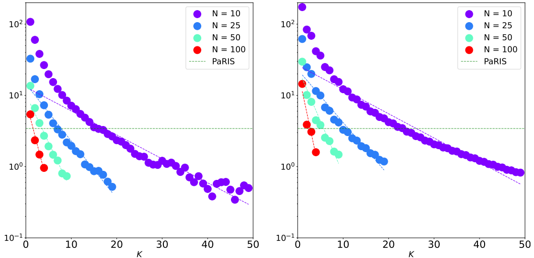
Figure 3: Output of the PPG roll-out estimator for the LGSSM. The curves describe the evolution of the bias with increasing k for different particle sample sizes N . The left and right panels correspond to k_0 = k - 1 and k_0 = \lfloor k/2 \rfloor , respectively.
