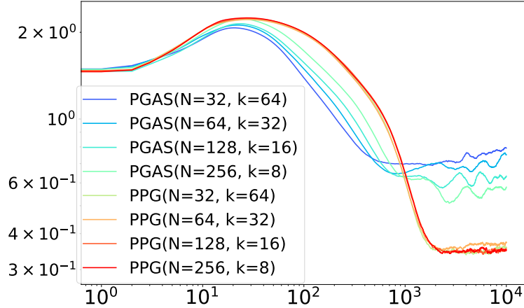
Figure 2: Distance to the MLE estimator as a function of the iteration step for PGAS and PPG with different parameters while keeping the particle budget fixed for LGSSM for 25 different seeds.
