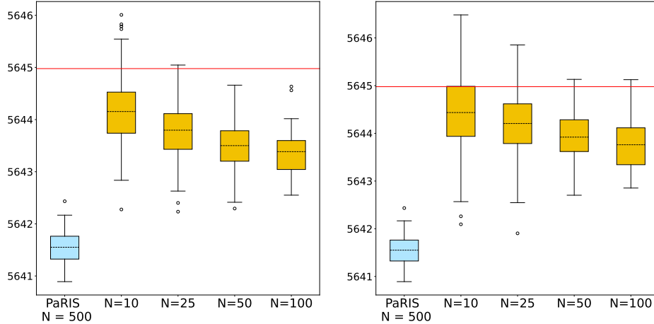
Figure 1: PARIS and PPG outputs for the LGSSM for C = 500 , yellow boxes correspond to PPG outputs produced using k \in \{50, 20, 10, 5\} iterations and N \in \{C/50, C/20, C/10, C/5\} particles. The image on the left corresponds to taking k_0 = k/2 and the one on the right to k_0 = k/4 .
