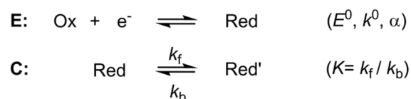
Scheme 2. EC mechanism with associated constants.
