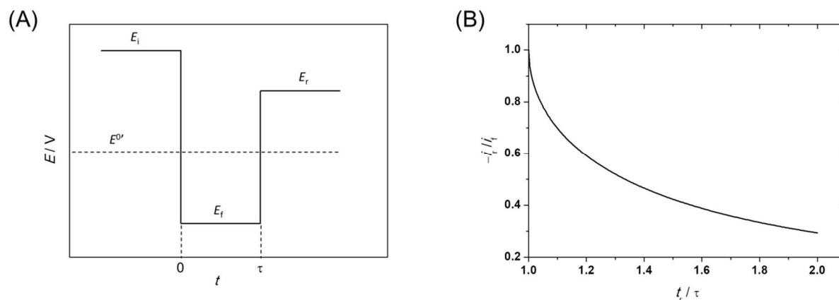
Figure 4. A) General waveform for a double potential step experiment for a reduction process and B) resulting variation of -i_r/i_f vs. t_r/\tau .
