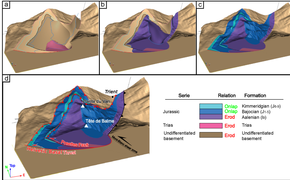
Fig. 11. Views of 3D GeoModel, from the central part of the synclinorium: the Montagne des Posettes. a) to d), views of the GeoModel with the different layers removed. The basal decollement and the Posettes thrust are highlighted in red. The Mont-Blanc shear zone is not modeled here, however, its position is shown in the Fig. . The stratigraphic pile of the model as well as the relationship between them is shown in d.
